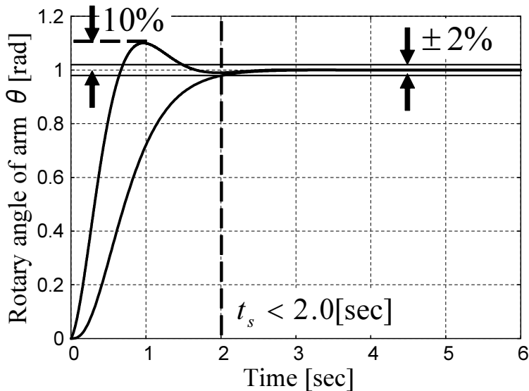
Fig. 6. Time domain performance specification
