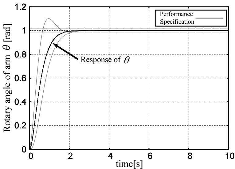
Fig. 11. Simulation result with QFT
