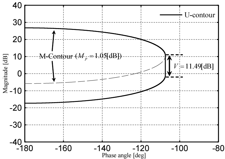
Fig. 9. U-contour on NC
