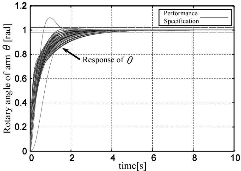
Fig. 12. Simulation result with PID
