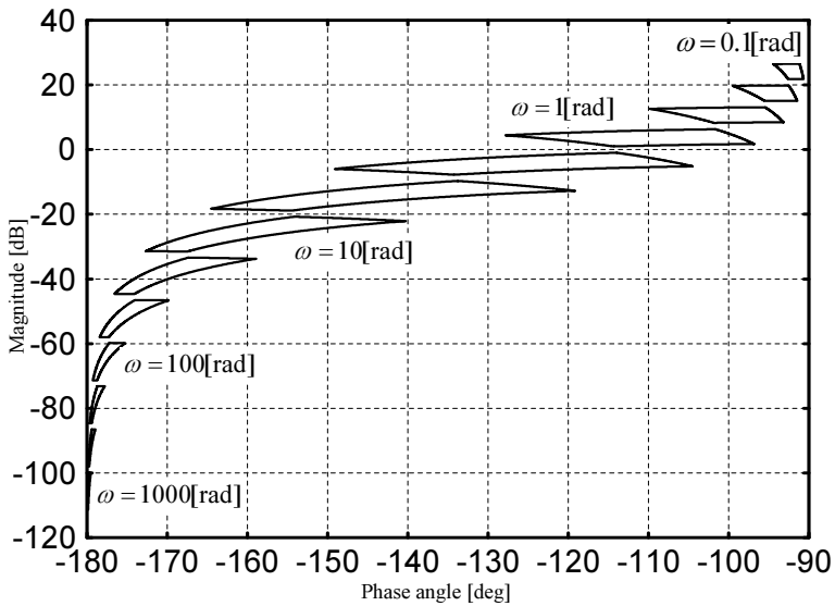
Fig. 8. Plant's template on NC
