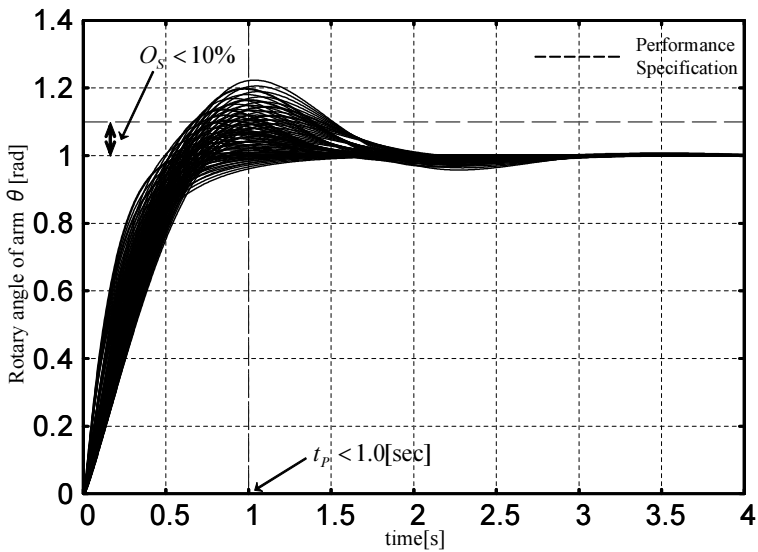
Fig. 4. Simulation result for \mathcal{P}(s)
