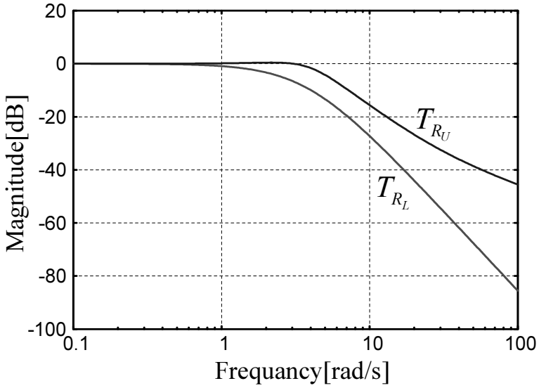
Fig. 7. Frequency domain performance specification
