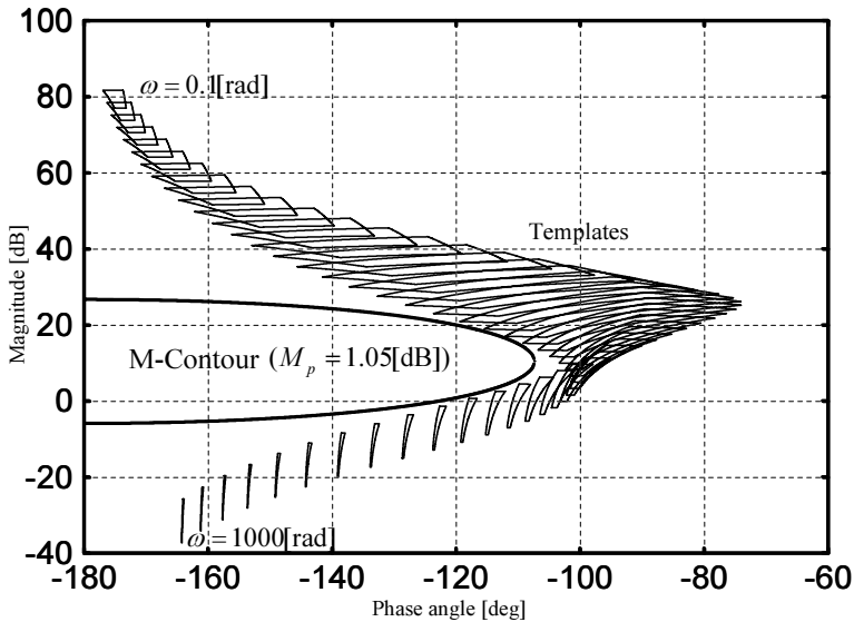
Fig. 10. M-contour and templates on NC
