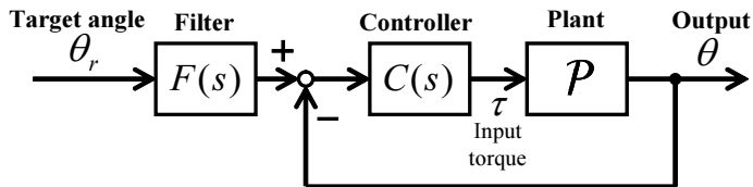
Fig. 5. QFT Control System
