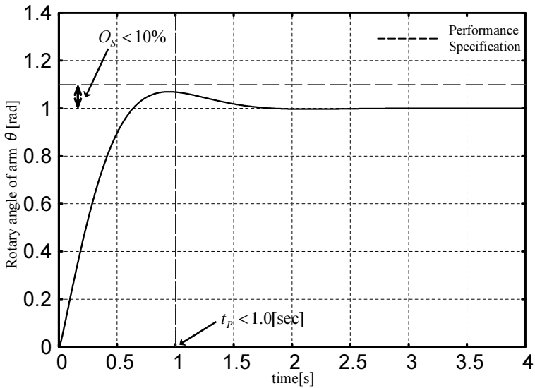
Fig. 3. Simulation result for \bar{P}(s)
