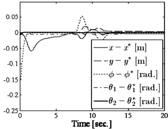
Fig. 5. Position tracking errors
