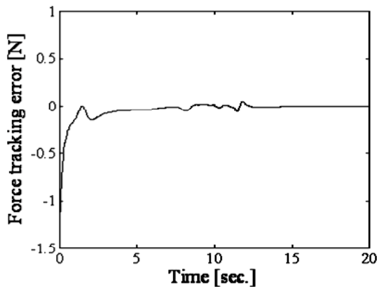
Fig. 6. Force tracking error
