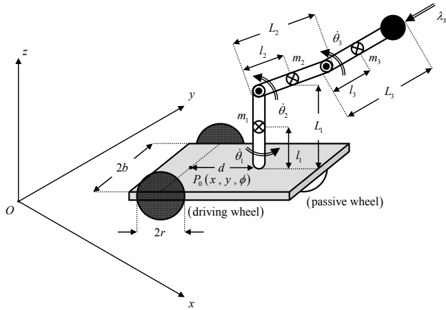
Fig. 3. Mobile manipulator used for simulations and experiments
