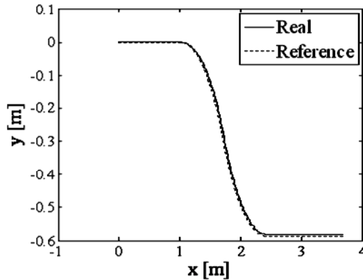
Fig. 4. Trajectory on (x, y) plane
