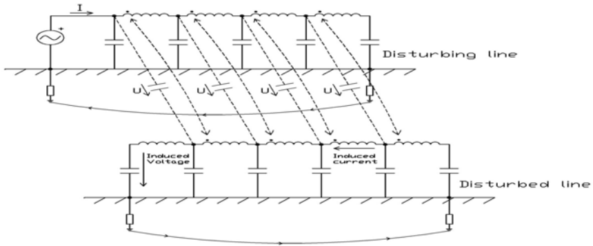
Fig. 1. Coupled inductors and coupled capacitors between the disturbing line and the disturbed line
