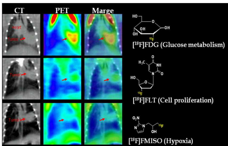
Fig. 2. PET, CT, and combined PET/CT-images of orthotopic human lung tumor xenografts in mice. Mice were administrated via the tail vein 15 MBq of [^{18}\text{F}] -FDG for detection of glucose metabolism (top row), [^{18}\text{F}] -FLT for detection of cell proliferation (middle row) and [^{18}\text{F}] -FMISO for detection of hypoxia (bottom row). PET images were acquired for 50 to 60 min after tracer administration using three-dimensional ordered subset expectation maximization (3D-OSEM) reconstruction.
