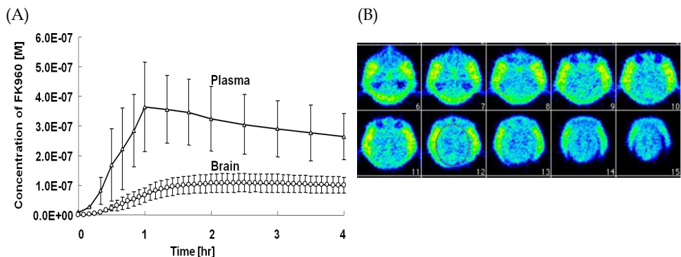
Fig. 3. (A) Brain and plasma concentrations of FK960 versus time in conscious male monkeys ( n=3 ) after oral administration of a mixture of 0.1 mg/kg of FK960 and 370 MBq tracer of [ ^{18}\text{F} ]-FK960 in saline. Concentrations of the drug into the entire brain were obtained from PET data. (B) Transverse PET images showing distribution of [ ^{18}\text{F} ]-FK960 into the brain. PET images were taken 90-120 min after drug administration as 3.6 mm transverse slices from the lower brain (top left) to the upper brain (bottom right). FK960 reached higher concentrations in the lower brain compared to the upper brain. The circle as presented in image 12 indicates the brain area in the skull.
