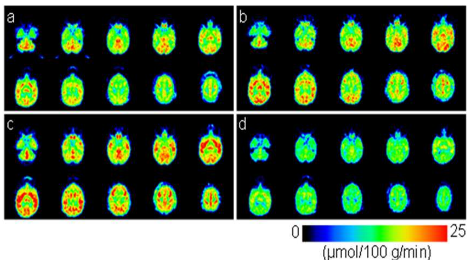
Fig. 5. PET images of the brain of conscious monkeys demonstrating rCMRglu using FDG-PET after treatment with empty vehicle (a), donepezil 500 µg/kg (b), scopolamine 30 µg/kg (c), and donepezil+scopolamine (d). Images are orbitomeatal transverse slices (OM) + 0 to OM + 32.4 mm, 3.6 mm thick.
