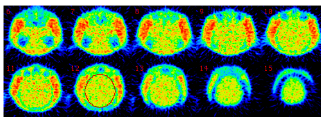
Fig. 8. (A) Correlations between FK-962 drug concentrations in plasma and the brain in monkeys and humans using PET imaging. (B) Transverse PET images showing distribution of [ ^{18}\text{F} ]-FK9602 in the brain of conscious monkeys. PET images were taken 90-120 min after drug administration as 3.6 mm transverse slices from the lower brain (top left) to the upper brain (bottom right). The circle as presented in image 12 indicates the brain area in the skull.
