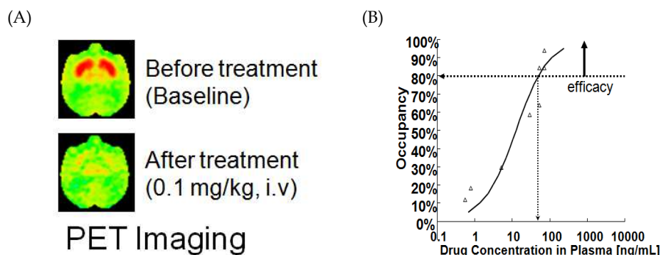
Fig. 4. (A) PET images of [ ^{11}\text{C} ]-SCH442416 before and after treatment of adenosine A_{2A} receptor antagonist, ASP5854, in conscious monkeys. At baseline, the tracer accumulated in the striatum, which is rich of A_{2A} receptors (20 mCi, i.v. injection; mean of six animals). At t=1\text{h} after drug administration (0.1 mg/kg, i.v.), the accumulation of the tracer in the striatum was lower compared to baseline, due to decreased binding of the PET tracer to the receptor as a result of ASP5854 binding to the receptor. (B) Relationship between the dose and receptor occupancy at 1 h after drug administration. Sigmoidal dose-response curve demonstrating an increase in adenosine A_{2A}R occupancy by ASP5854 with an increase in ASP5854 plasma concentration at t=1\text{h} after drug administration (dose-levels: 0.001 to 0.1 mg/kg, i.v.); 80% receptor occupancy correlated with efficacy (catalepsy) in the monkeys.
