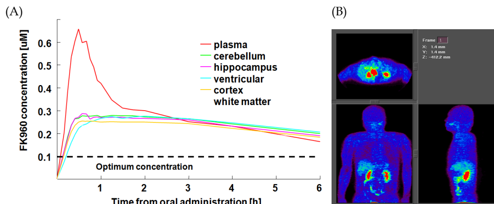
Fig. 7. (A) Concentration versus time curves of FK-960 in plasma and different area's of the brain in healthy subjects following oral administration of a mixture of [ ^{18}\text{F} ]-FK960 and FK960 (6mg, n=3). (B) Biodistribution of [ ^{18}\text{F} ]-FK960 in human whole-body using PET imaging. Images were acquired 120-130 min after administration.
