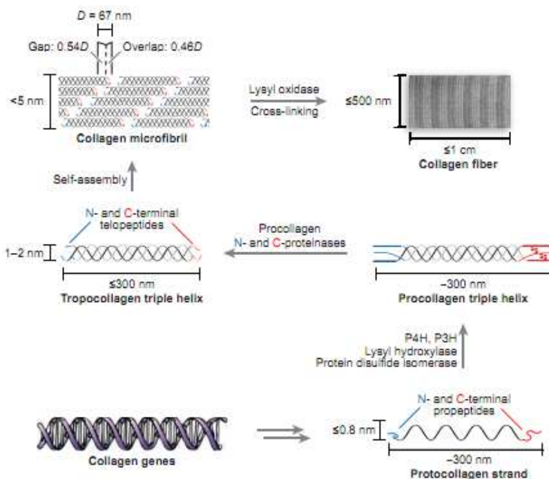
Fig. 1. Biosynthetic route of collagen fibers (Shoulders & Raines, 2009)
