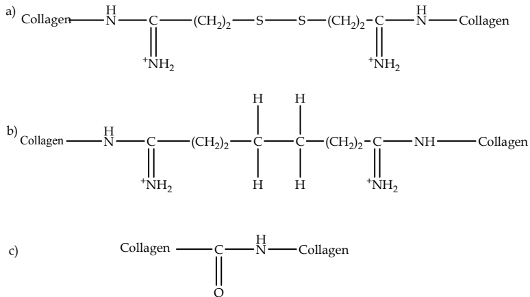
Fig. 8. Structure of cross-links obtained by (a) DTBP, (b) DMS and (c) acyl azide treatments (Charulatha & Rajaram, 2003).
