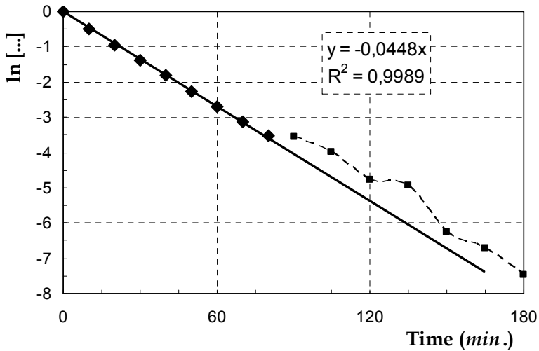
Fig. 15. Evaluation of the module efficiency through Eq. (20); same data as Fig. 13
