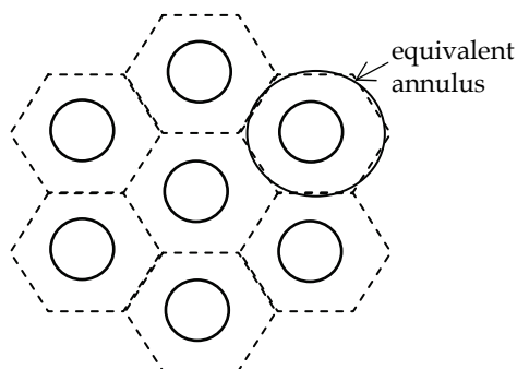
Fig. 8. The equivalent annulus approximation
