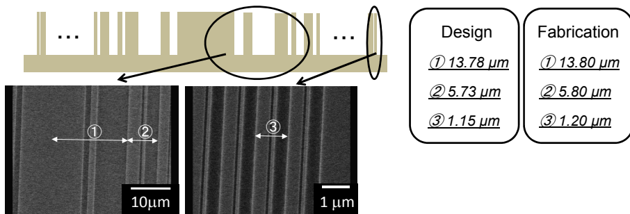
Fig. 9. SEM image of the fabricated binary convex diffractive lens with a 150- \mu\text{m} focal length ( N = 4 ) on the PET film
