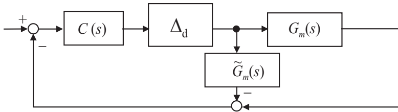
Fig. 8. Model based control structure
