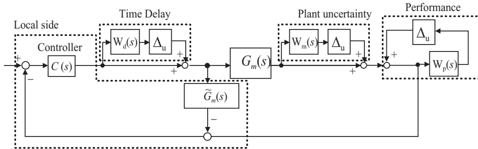
Fig. 9. Overall structure with perturbations
