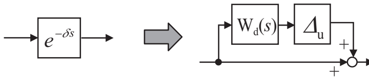
Fig. 7. Time varying delay as a perturbation
