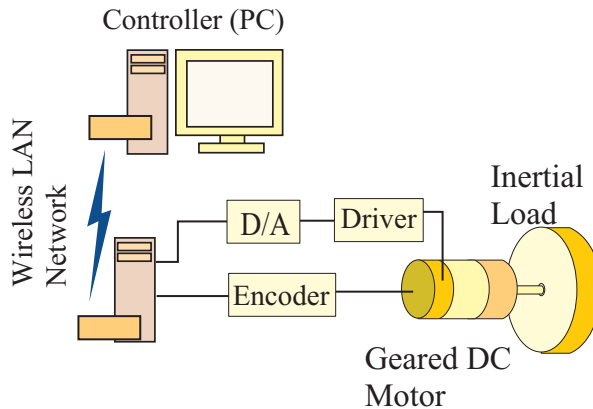
Fig. 12. Experimental setup and system configuration
