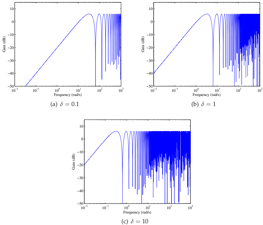
Fig. 3. Bode plot of e^{-\delta s} - 1
