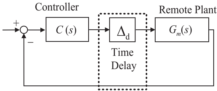
Fig. 6. Basic structure of network based system
