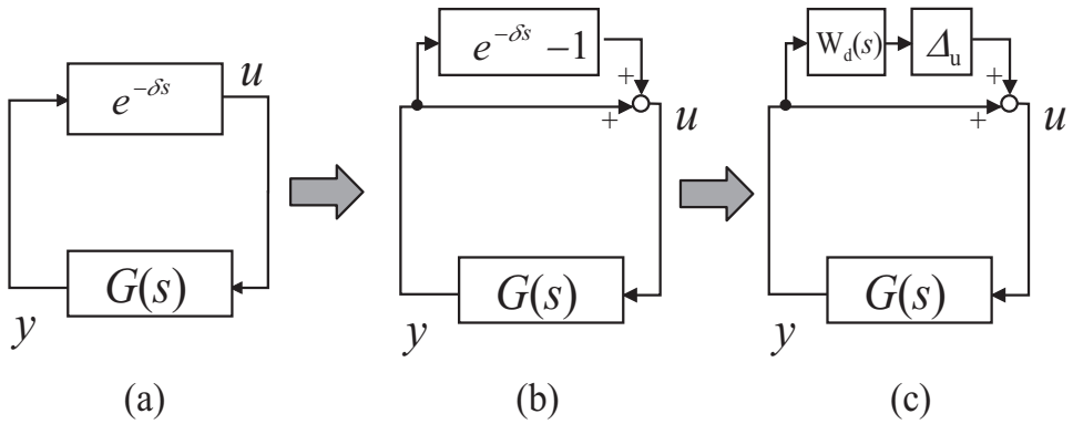
Fig. 2. Robust control based method
