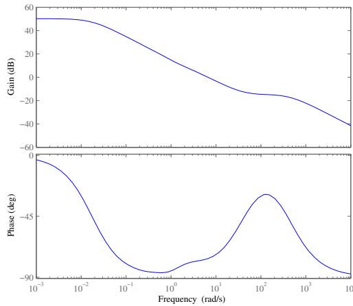
Fig. 15. Bode plot of the controller C(s)
