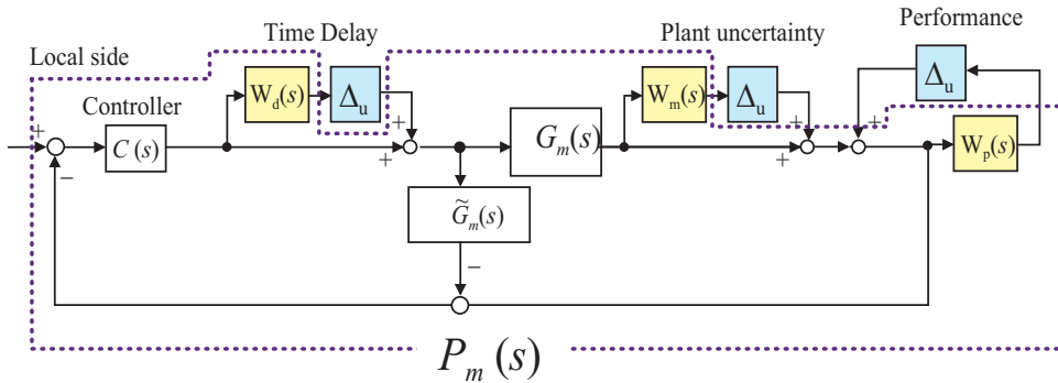
Fig. 10. Augmented plant P_m
