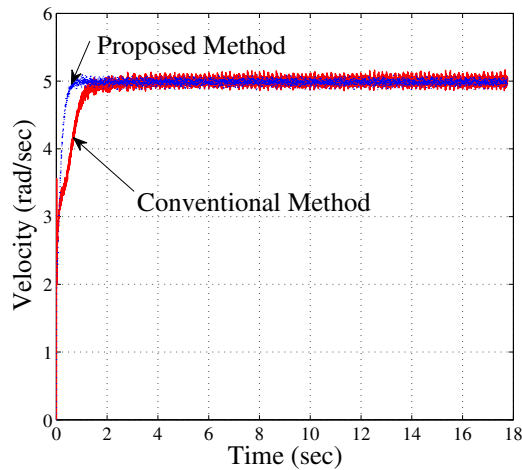
Fig. 17. Experimental results (Step response of velocity control)
