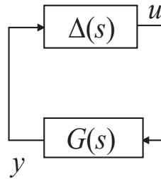
Fig. 1. Interconnection of a plant and time delay
