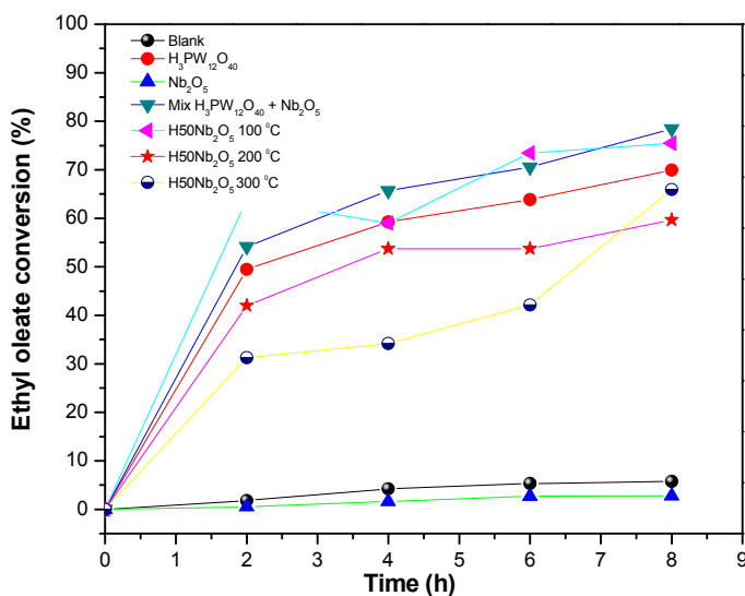
Fig. 6. H_3PW_{12}O_{40}/Nb_2O_5 -catalyzed oleic acid esterification with ethanol
