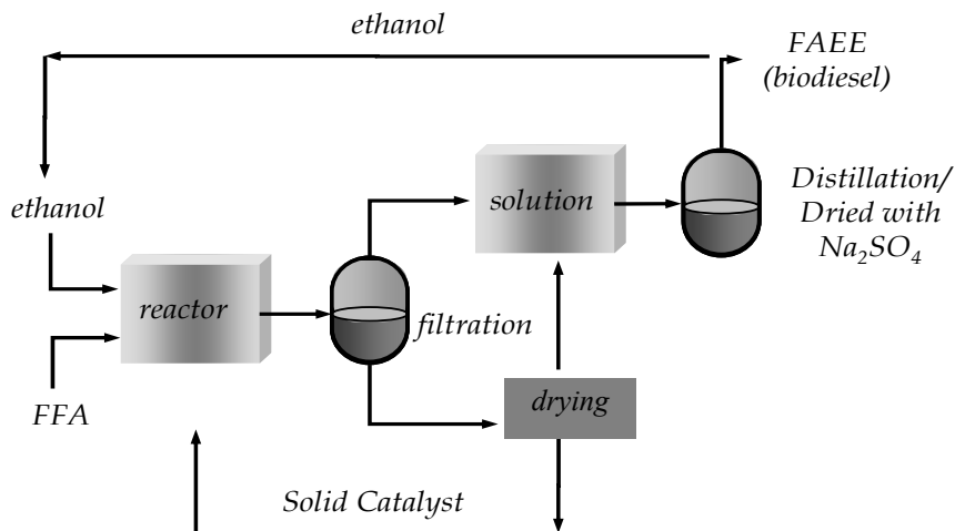
Fig. 4. Scheme of a typical acid solid-catalyzed process of FFA esterification in liquid phase
