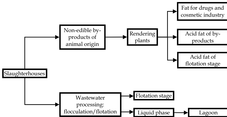
Fig. 5. Scheme of fat processing in slaughterhouses.
