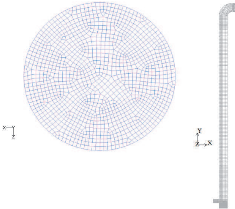
Fig. 2. Computational grid
