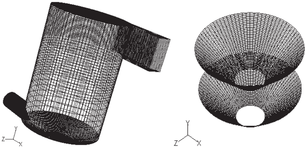
Fig. 4. Computational grid
