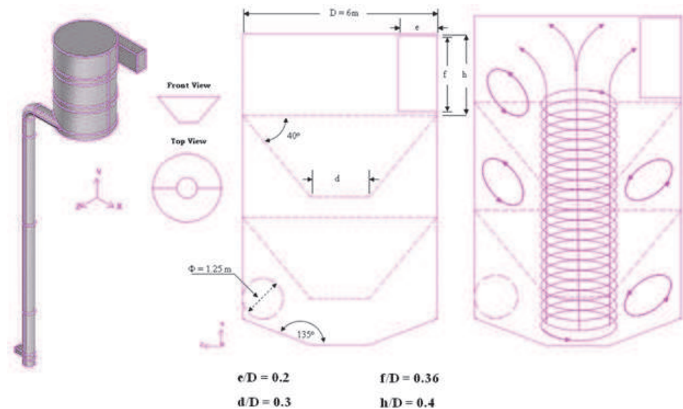
Fig. 3. Schematic of the pneumatic-cyclone dryer assembly
