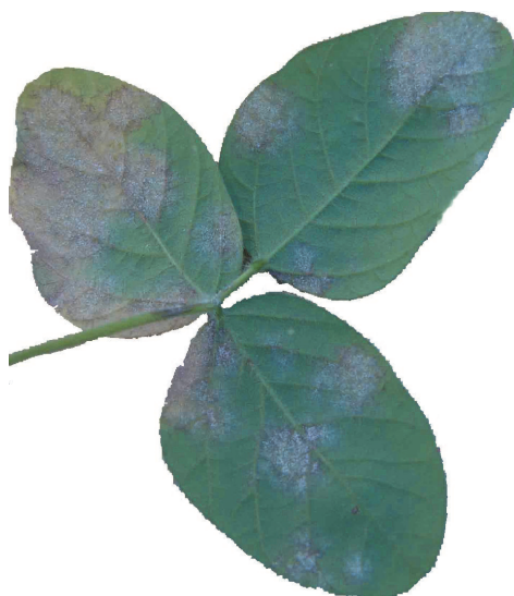
Fig. 1. Evaluated signals of powdery mildew in soybean plants.
