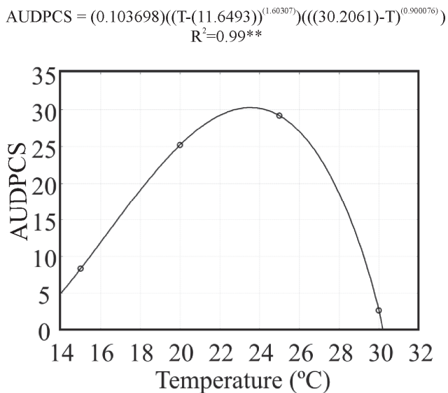
Fig. 4. Nonlinear regression of the progress curve of disease severity (AUDPCS) of powdery mildew of soybean in suprema cultivar according to the isolated effect of temperature.
