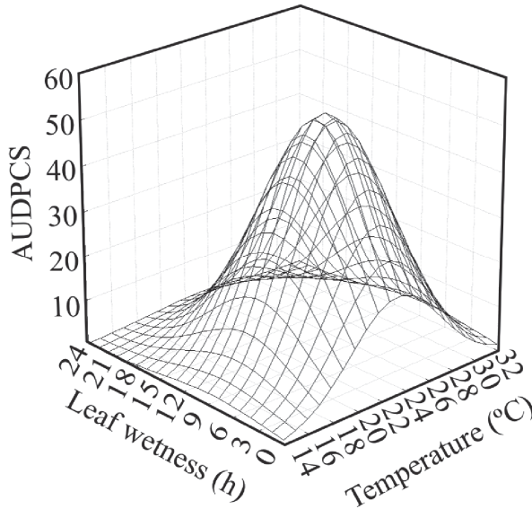
Fig. 2. Nonlinear regression of the progress curve of disease severity (AUDPCS) of powdery mildew of soybean in conquista cultivar according to the interaction between temperature and leaf wetness.
