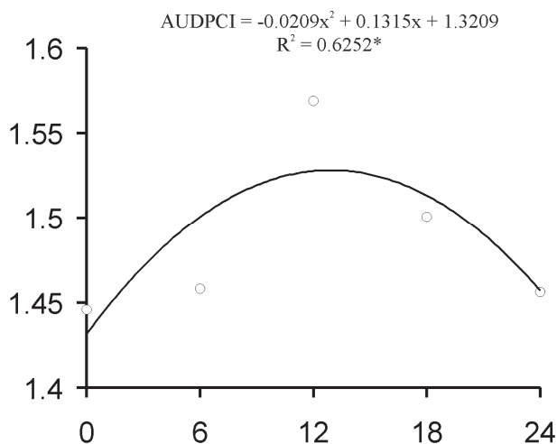
Fig. 5. Linear regression with polynomial quadratic fit of the progress curve of disease incidence (AUDPCI) of powdery mildew of soybean in suprema cultivar (Y axis) according to the isolated effect of leaf wetness (X axis).
