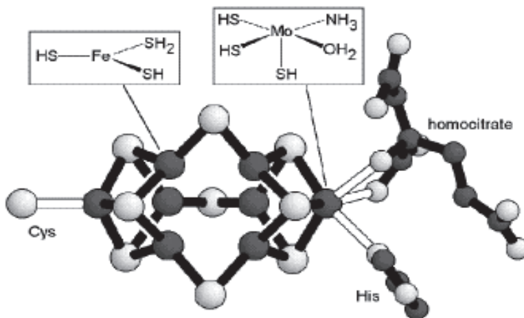
Fig. 6. Structure of nitrogenase enzyme (Durrant, 2001)
