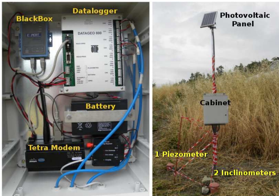
Fig. 4. Cabinet and installation site
