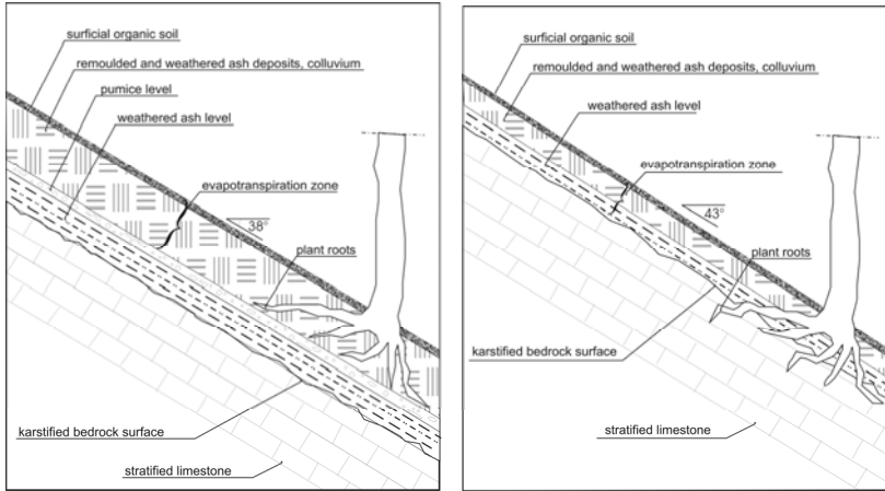
Fig. 2. Schematic profile of a typical slope of high-elevated zones of the Campania region (overlapping and thickness of the levels are schematised). Pumice levels limit plant roots development in the upper zone of the soil mantle (left); plant roots reach the karst substratum if pumice levels are absent (right).
