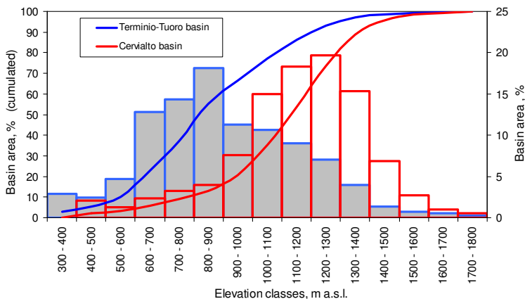
Fig. 3. Elevation classes distribution of the Terminio-Tuoro and Cervialto basin.
