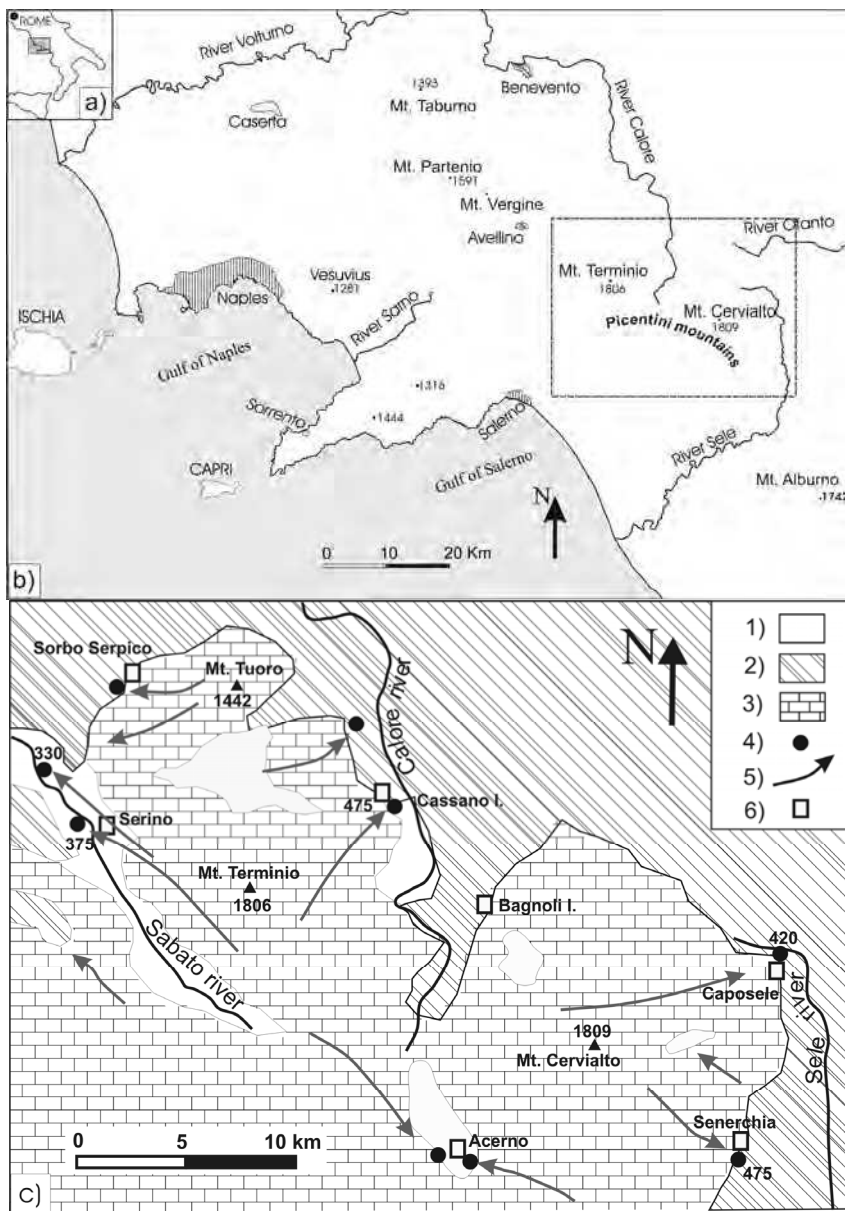
Fig. 1. a) Southern Italian peninsula. b) Map of the Western Campania region. Delimited rectangular area is detailed in c). c) Hydrogeological map of the Northern Picentini Mountains. 1) Slope breccias and debris, pyroclastic, alluvial and lacustrine deposits (Quaternary); 2) argillaceous complex and Flysch sequences (Paleogene–Miocene); 3) calcareous-dolomite series (Jurassic–Miocene); 4) main spring; 5) groundwater flow direction; 6) main village.
