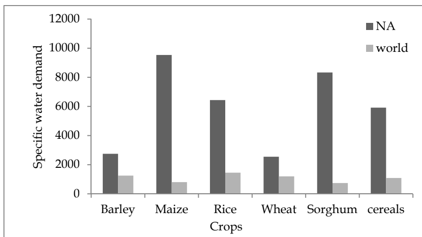
Fig. 6. Specific water demand for cereal crops in the North African and world (m 3 /ton) 2003-2007
