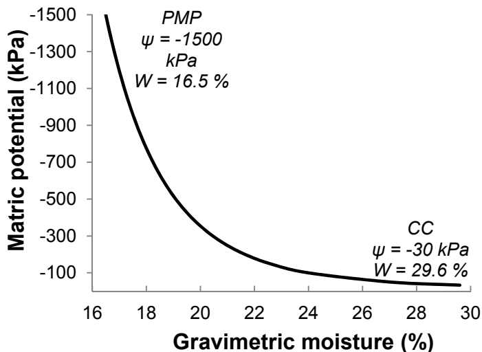
Fig. 3. Moisture retention curve in the experimental site.
