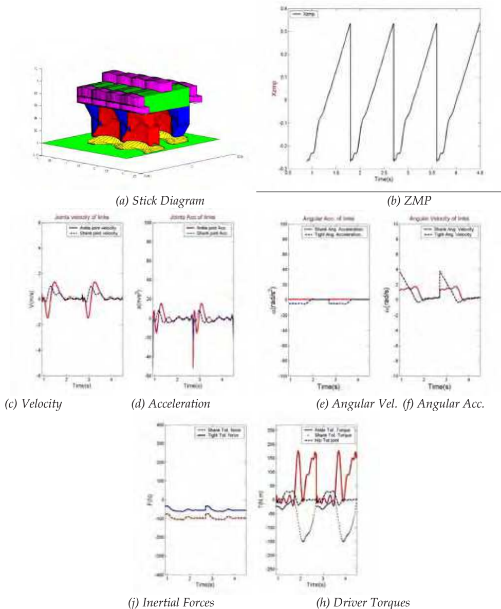
Fig. 1.8. (a) The robot's stick diagram on \lambda = 0^\circ , Moving ZMP, H_{\min} = 0.60m, H_{\max} = 0.62m (b) The moving ZMP diagram in nominal gait which satisfies stability criteria (c) \_ : Shank M.C velocity, \_ : Tight M.C velocity (d) \_ : Shank M.C acceleration, \_ : Tight M.C acceleration (e) \_ : Shank angular velocity, \_ : Tight angular velocity (f) \_ : Shank angular acceleration, \_ : Tight angular acceleration (g) \_ : Shank M.C inertial force, \_ : Tight M.C inertial force (h) \_ : Ankle joint torque, \_ : Hip joint torque, \dots : Shank joint torque
