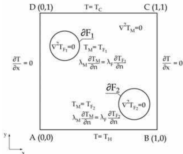
Fig. 1. Composite elementary cell structure
