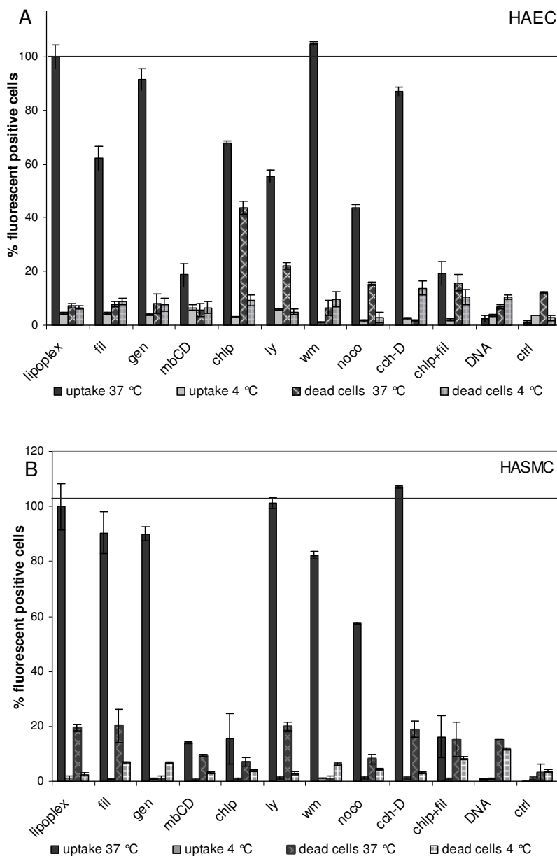
Fig. 1. Cells were incubated for one hour with Cy-5 labeled lipoplexes and analyzed by means of flow cytometry (FL-4 channel). Prior to the measurement, every sample was additionally incubated with 7-AAD to determine the amount of dead cells (FL-3 channel). Error bars indicate standard deviation (n=3 in 3 independent experiments).
