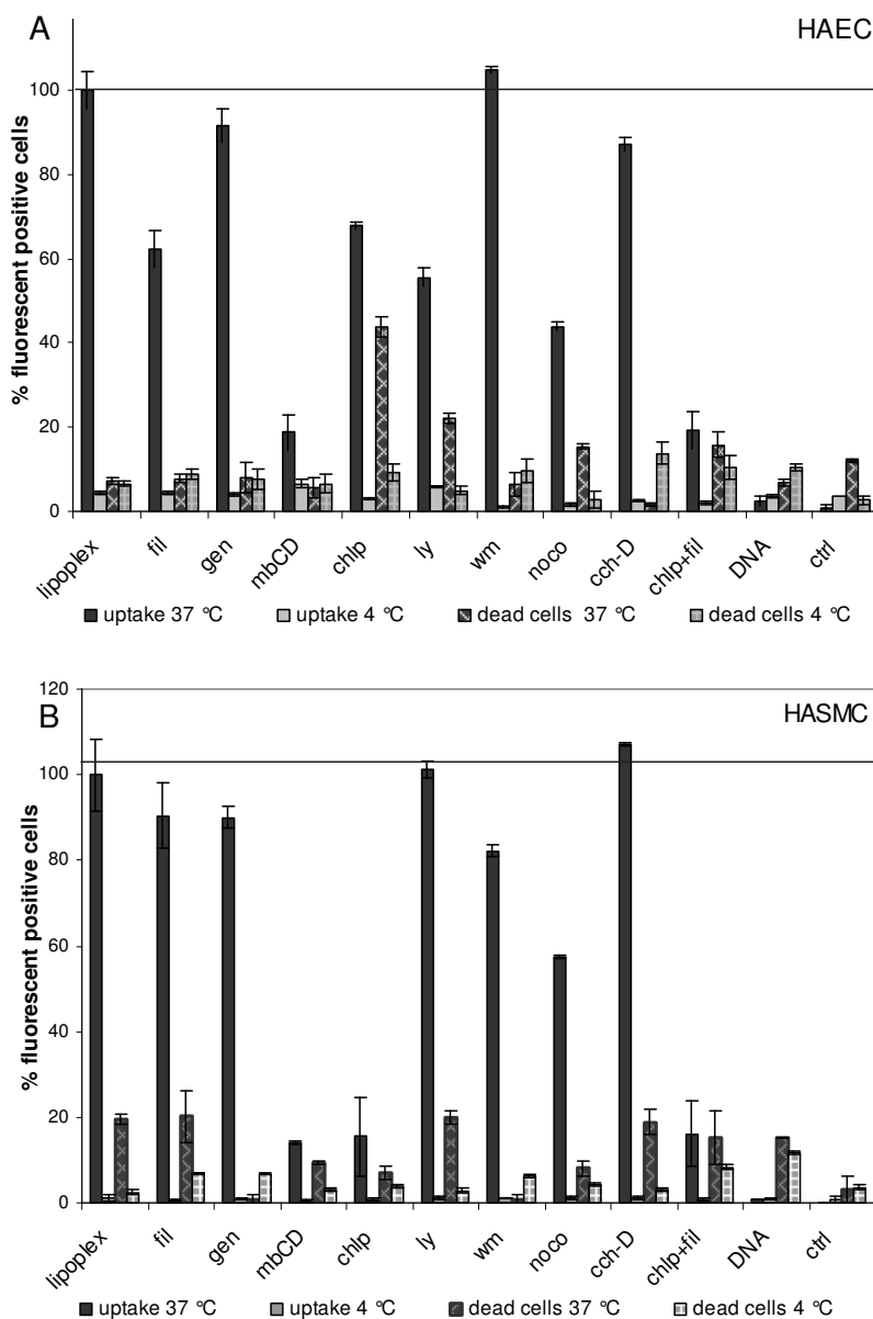
Fig. 2. After pre-incubation with different inhibitors (see Table 1) (x-range), HAEC (A) and HASMC (B) were incubated for one hour with Cy-5 labeled DC-30® lipoplexes and analyzed by means of flow cytometry (FL-4 channel). Prior to measurement, every sample was also incubated with 7-AAD to determine the amount of dead cells (FL-3 channel). The fluorescence intensity of lipoplexes without inhibitors was set to 100%. Error bars indicate standard deviation (n=3 in 3 independent experiments).
