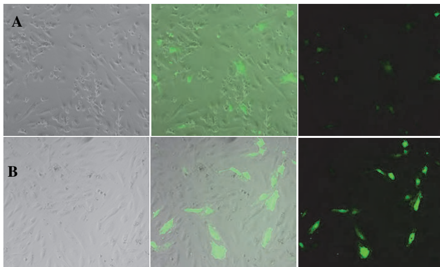
Fig. 6. HAEC (A) and HASMC (B) after electroporation of pEGFP and 48 h incubation. Left-handed: brightfield; Right handed: fluorescent picture (GFP), middle position: overlay of pictures.
