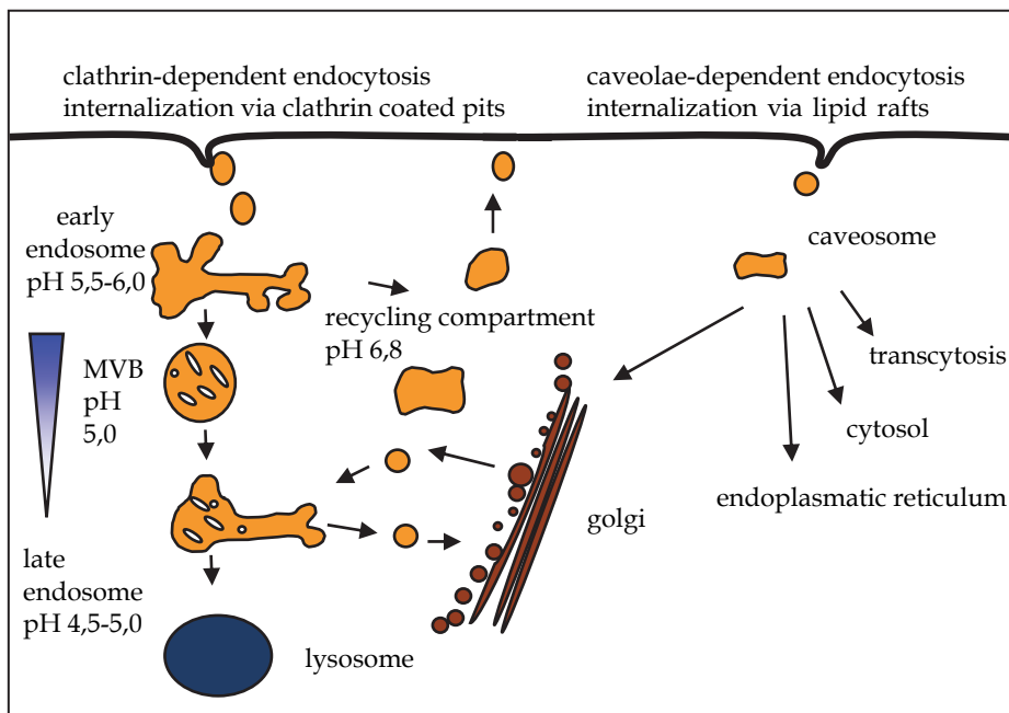
Fig. 5. Cartoon of the main cellular internalization routes of lipoplexes. On the left hand the clathrin-dependent pathway and on the right hand the caveolae-mediated uptake mechanisms are shown. Whereas the first pathway has been well investigated, caveolin-mediated internalization has not been examined in detail to date. The first step in the clathrin-dependent pathway is the budding of clathrin-coated vesicles resulting in early or sorting endosomes. Recycling back to the membrane happens in recycling endosomes. Early endosomes transform in MVB and subsequently late endosomes are formed which end up as lysosomes. Active exchange between the golgi apparatus and late endosomes is known. Particles, internalized via caveolae from so-called caveosomes offering various processing possibilities such as transcytosis, cytosolic release, delivery to the ER or transport to the golgi apparatus.
