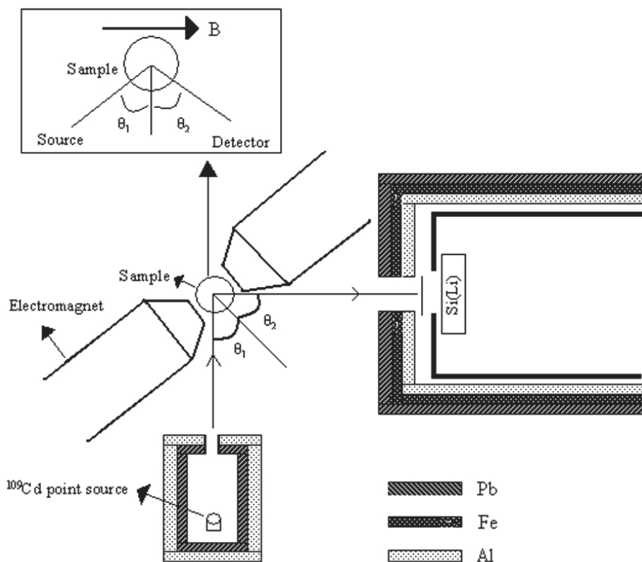
Fig. 1. Experimental set-up.
