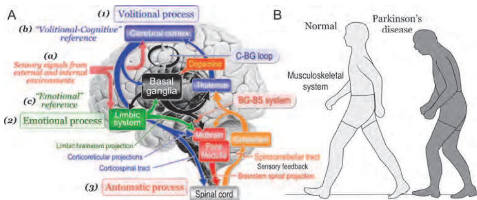
Fig. 1. Fundamental signal flows involved in gait control
