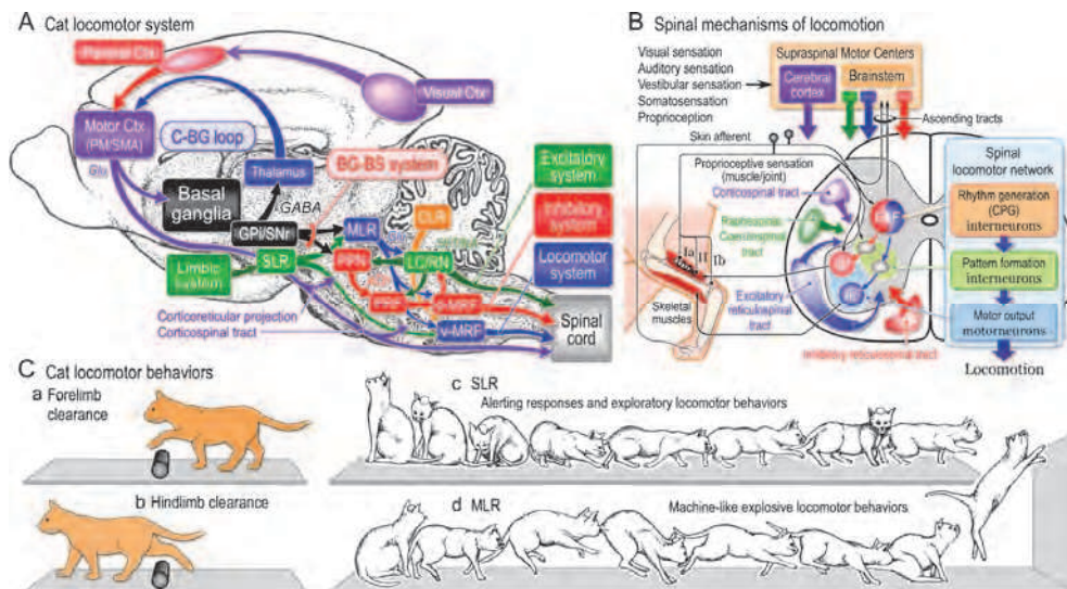
Fig. 3. Neuronal mechanism of locomotion in cats
