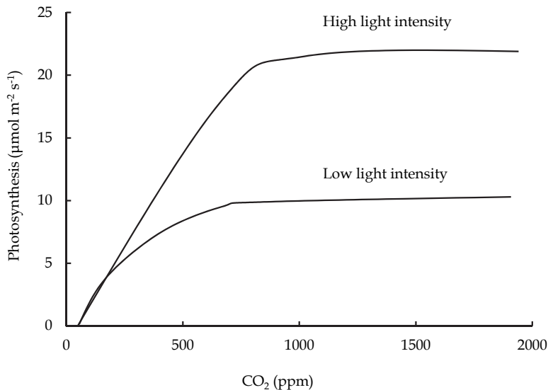
Fig. 1. Photosynthetic curves at high and low light intensities.
