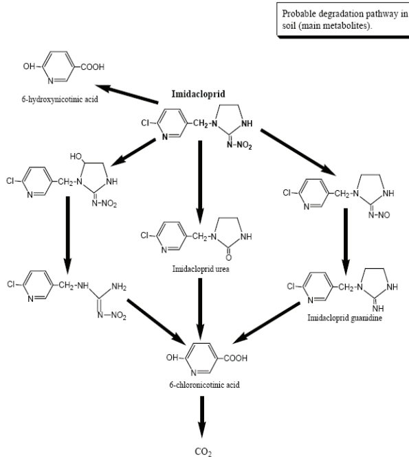
Fig. 3. The proposed metabolic pathway of IMI in the soil.
