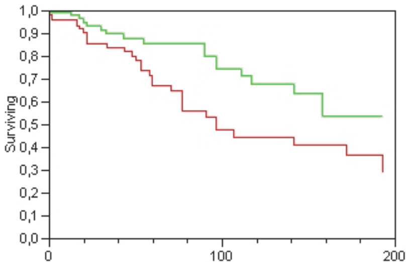
Fig. 3. Survival rates of the two groups with the Kaplan-Meier method (SAS 2002)
