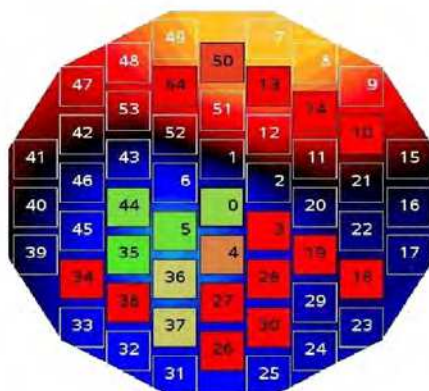
Fig. 5. Magnetic field map with channels position: The different colors of the channels correspond to different values of FI from green (low FI) to red (high FI): the transparent channels correspond to unused channels since too noisy (i.e 29) or too close to the 0 line (i.e: 1).
