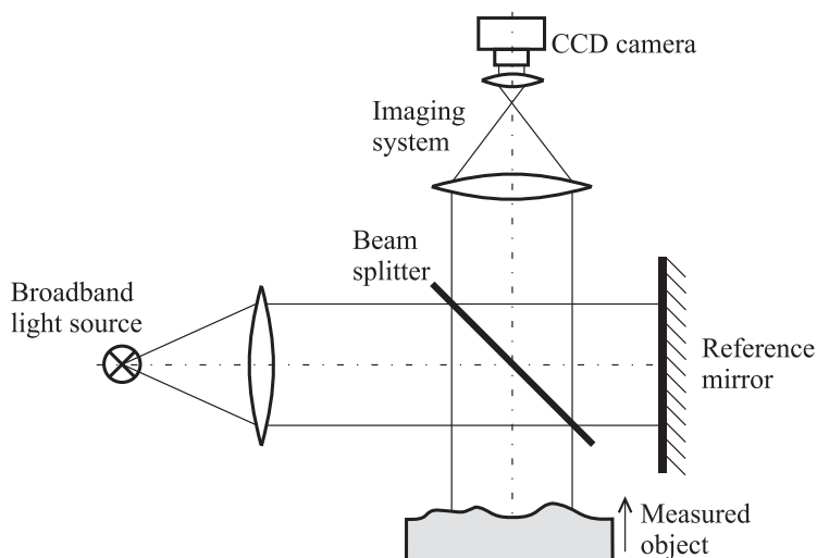
Fig. 1. Schematic of white-light interferometry.
