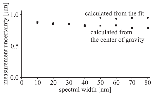
Fig. 8. Numerically calculated measurement uncertainty \delta z as a function of spectral width \Delta\lambda for \lambda_0 = 820nm , \sigma_h = 1.2\mu m , I_{\text{obj}} = \langle I_{\text{obj}} \rangle , and NSR = 0.05 .
