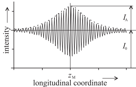
Fig. 2. Typical white-light correlogram.
