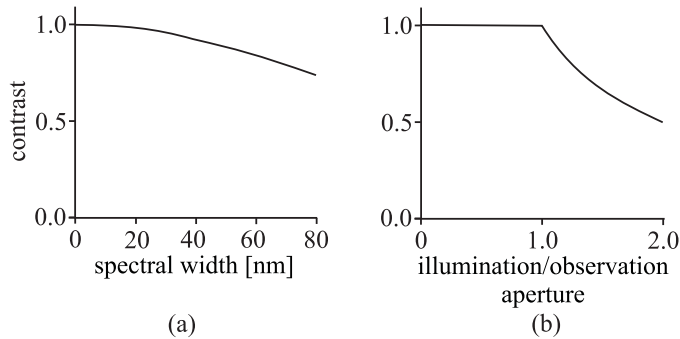
Fig. 6. (a) Speckle contrast as a function of spectral width (numerically calculated data) for \lambda_0 = 820\text{nm} , \sigma_h = 1.2\mu\text{m} . (b) Speckle contrast as a function of illumination aperture according to Häusler.
