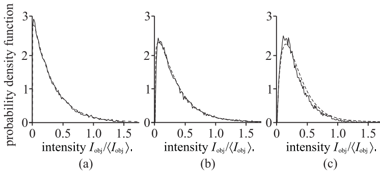
Fig. 5. Intensity distribution for \lambda_0 = 820nm, \sigma_h = 1.2\mu m . (a) \Delta\lambda = 10nm . (b) \Delta\lambda = 38nm . (c) \Delta\lambda = 80nm .
