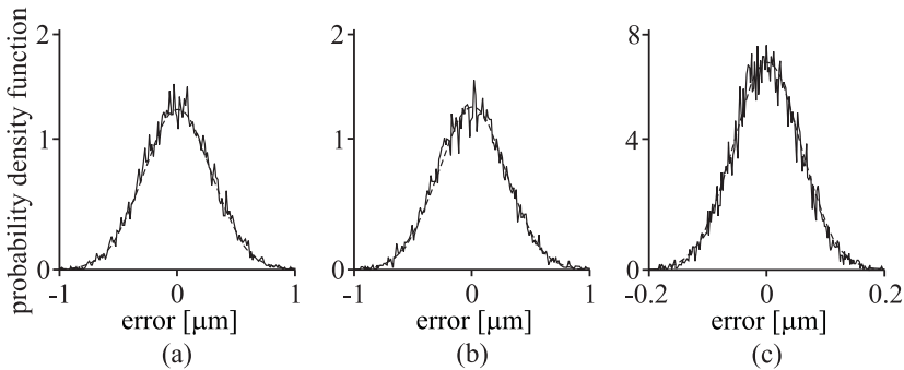
Fig. 7. Distribution of the measurement error for \lambda_0 = 820\text{nm} , \Delta\lambda = 35\text{nm} , \sigma_h = 0.4\mu\text{m} , I_{\text{obj}} = \langle I_{\text{obj}} \rangle , and \text{NSR} = 0.05 . (a) Error caused by surface roughness and shot noise. (b) Error caused by surface roughness only. (c) Error caused by shot noise only.
