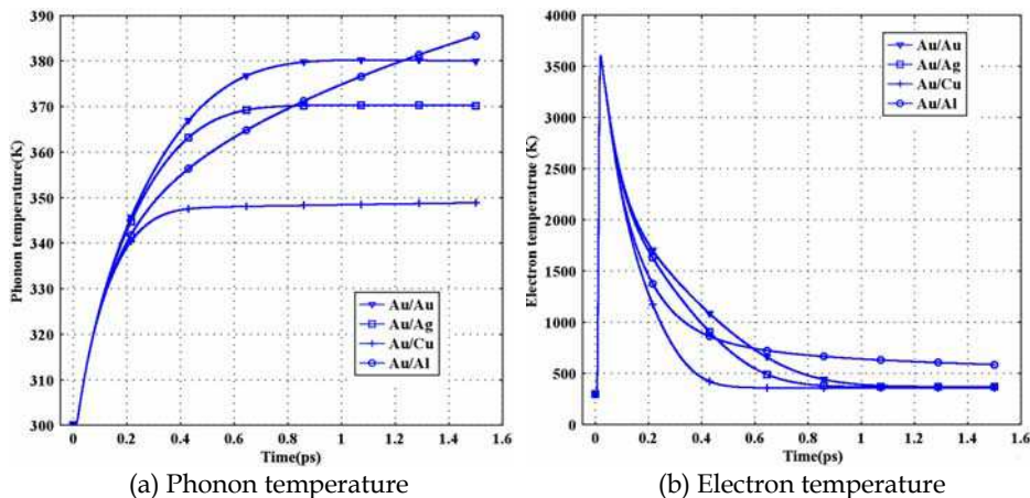
Fig. 6. Temporal evolution of phonon and electron temperatures at center of laser spot on surface of Au surfaced two layer metal film assemblies
