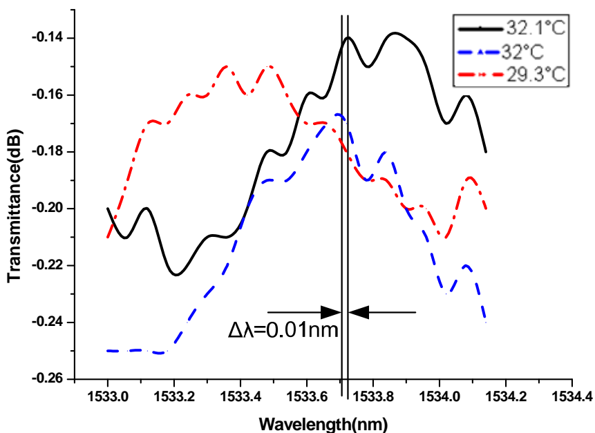
Fig. 12. Wavelength lock.
