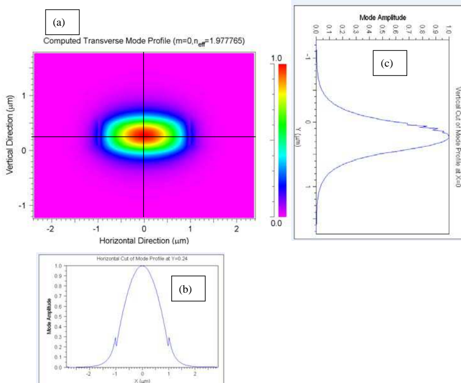
Fig. 4. Simulated fundamental mode profile from BPM-based calculations.
