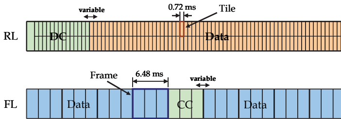
Fig. 10. Multi-Frame structures.
