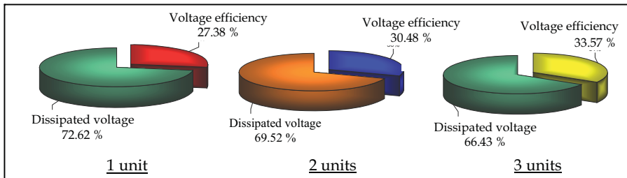
Fig. 22. Pie chart for sample capacitor 0.68µF (CBB20)
