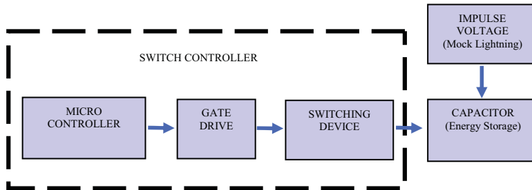
Fig. 4. Block diagram of the high speed switching circuit
