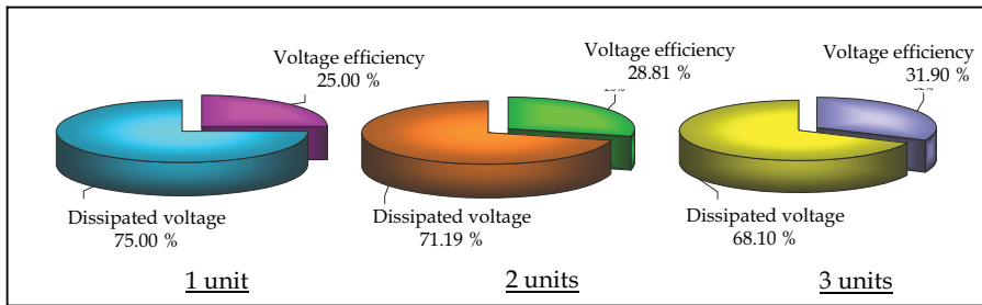
Fig. 21. Pie chart for sample capacitor 0.47µF (CBB20)
