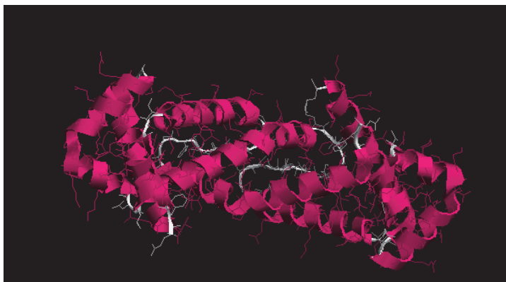
Fig. 7. Structure of SRP 54 (Gowda et al., 1998).
