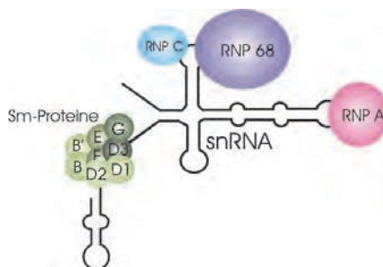
Fig. 9. Schematic view of the snRNP.
