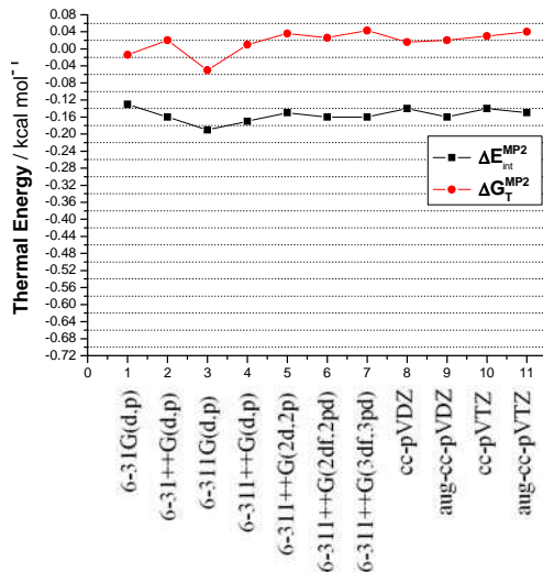
Fig. 2. Anti → gauche MP2 thermal energy variation (at room temperature) for 1,2-difluorethane as a function of the basis set quality. The MP2/6-311++G(3df,3pd) and MP2/aug-cc-pVTZ \Delta S values (entropic contribution) are respectively -0.20 and -0.19 kcal mol -1 (see Eq. 2).
