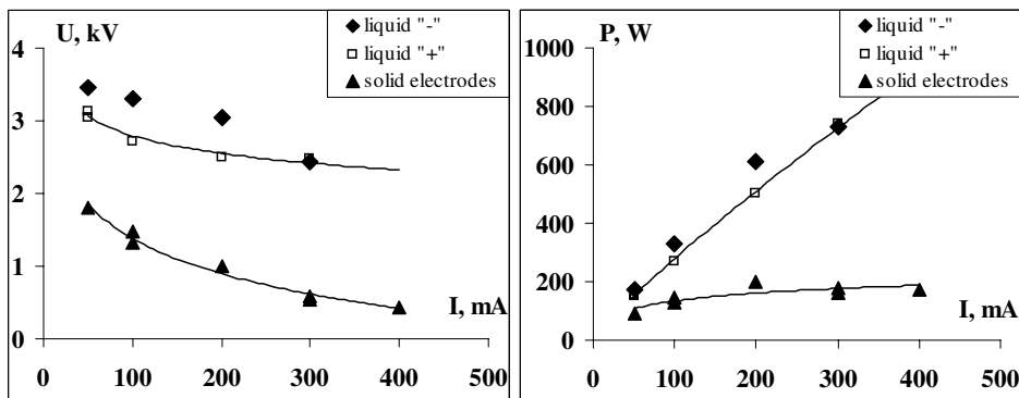
Fig. 15. Current-voltage (left) and power (right) characteristics of the DGCLW working in different modes in ethanol-water solution (5/1). Air flow rate G= 55 cm 3 /s.
