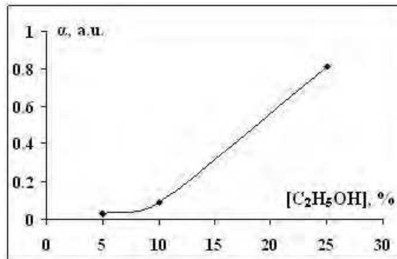
Fig. 33. Coefficient of energy transformation for the ethanol reforming in the TORNADO-LE as a function of the initial ethanol concentration.
