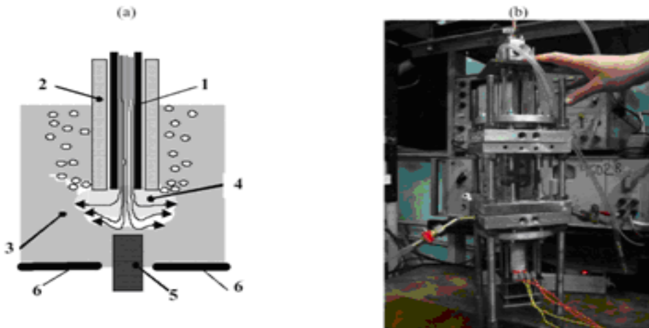
Fig. 3. DCGLW (dc) in the liquid with microbubbles induced by ultrasonic cavitation. (a) - Scheme of discharge with liquid electrode; (b) - photo of pulsed reformer.
