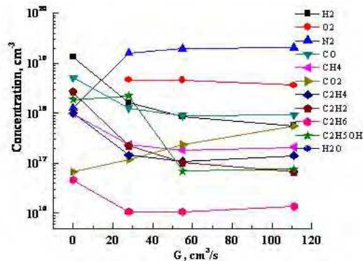
Fig. 18. Concentrations of output gas products after the ethanol processing in the DGCLW as function of air flow rate. Ethanol-water solution (5/1), I_d=100 \text{ mA} .
