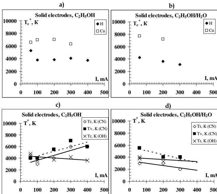
Fig. 13. Character temperatures T_e^*, T_r^*, T_v^* in discharge plasma vs. current in the DGCLW with solid electrodes: (a, c) are pure ethanol, (b, d) are ethanol/water mixture (5/1). Air flow rate G=55 \text{ cm}^3/\text{s} .
