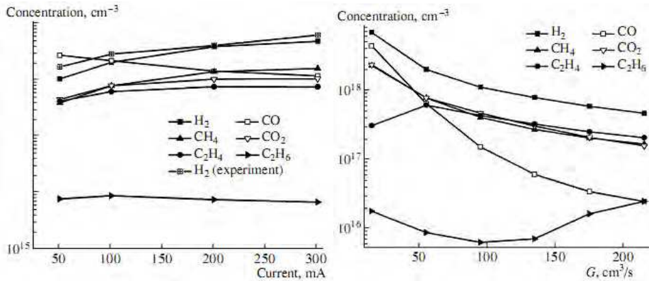
Fig. 19. Calculated concentrations of output gas products after the ethanol processing in the DGCLW as functions of discharge current (left, G = 55 \text{ cm}^3/\text{s} ) and air flow rate (right, I_d = 100 \text{ mA} ). \text{C}_2\text{H}_5\text{OH} : \text{H}_2\text{O} = 5:1 .
