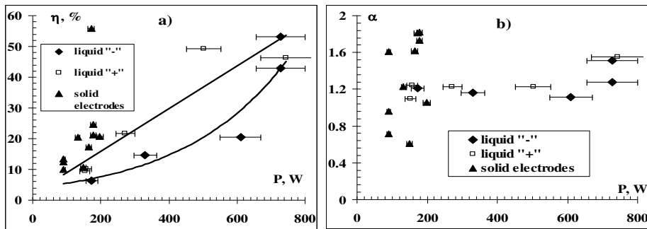
Fig. 20. Dependencies of (a) efficiency of conversion \eta and (b) coefficient of energy transformation \alpha for the ethanol reforming in the DGCLW in different discharge modes as a function of the discharge power (currents vary from 50 to 400 mA). C_2H_5OH : H_2O = 5:1
