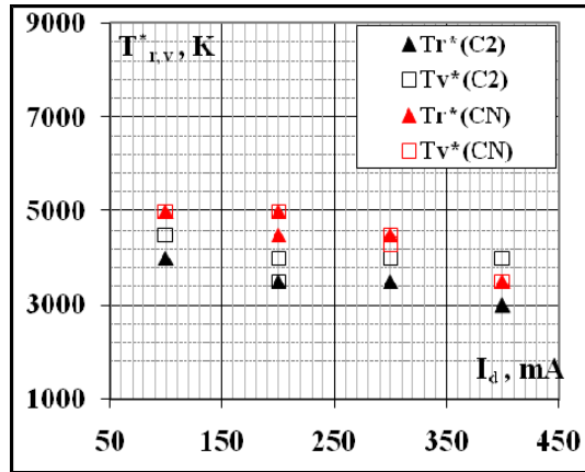
Fig. 12. Character temperatures T_r, T_v in discharge plasma vs. current in the DGCLW with the liquid anode working in ethanol/water mixture (5/1). Air flow rate G=55 \text{ cm}^3/\text{s} .
