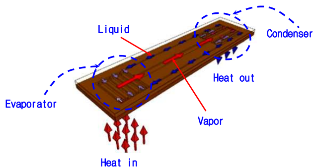
Fig. 18. An operating principle of the flat plate type micro CPL
