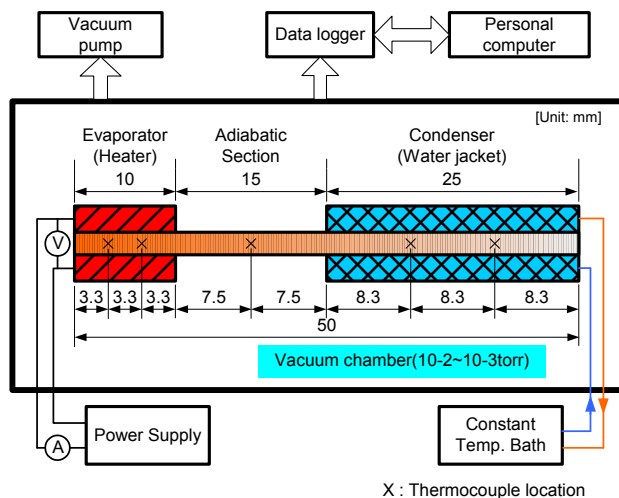
Fig. 6. Experimental apparatus
