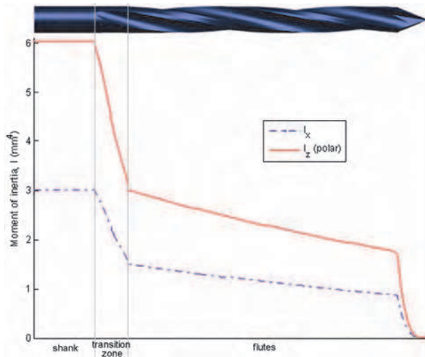
Fig. 9. I_x and I_z profiles for a 3-fluted drill-bit. (Bertollo, Gothelf et al. 2008)
