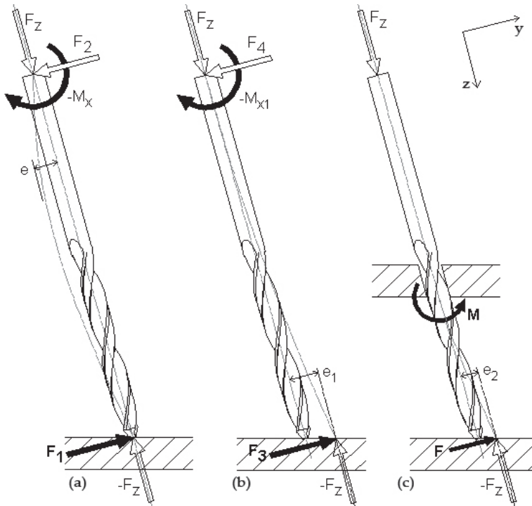
Fig. 6. Bending modes for a surgical drill. The deformation profile of the two-fluted drill-bit under each scenario is idealised and does not take into account the variation in second (area) moment of inertia properties along the length of the drill. (Bertollo, Gothelf et al. 2008)
