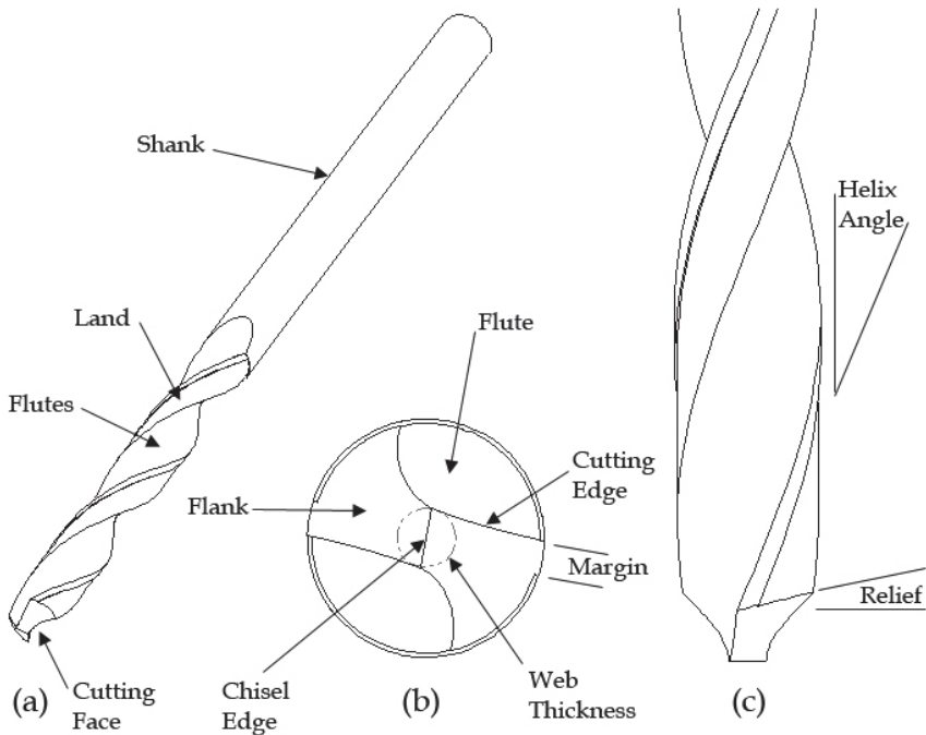
Fig. 2. Drill-bit geometry. (a) General geometry, (b) Point geometry, and (c) Relief and helix angles
