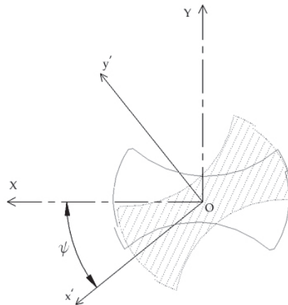
Fig. 7. Cross-section of a typical 2-fluted orthopaedic drill-bit. The second (area) moment of inertia of the fluted portion of the drill changes with rotation, \psi , of the cross-section relative to the global (x-y) coordinate system
