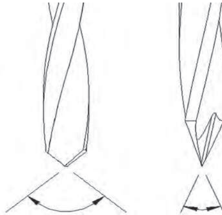
Fig. 4. Point angles of 2-fluted (left) drill-bits are generally less acute than for 3-fluted (right) surgical drill-bits. Web thickness at the tip of 2-fluted drill-bits limits the point angle which can be supported, as compared to the pyramidal shape of the 3-fluted tip
