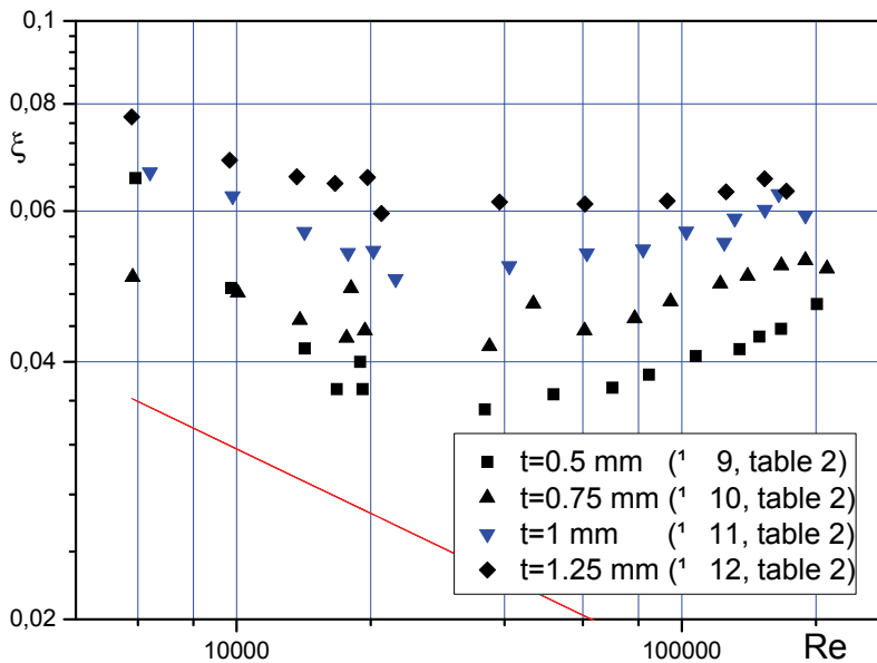
Fig. 17. Dependence of hydraulic resistance factor of rough tubes with rounded thread roughness profile on Re : line – for smooth tube (by calculation)
