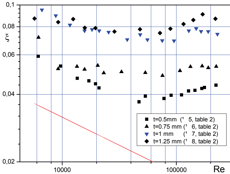
Fig. 16. Dependence of hydraulic resistance factor of rough tubes with rectangular thread roughness profile on Re : line – for smooth tube (by calculation)
