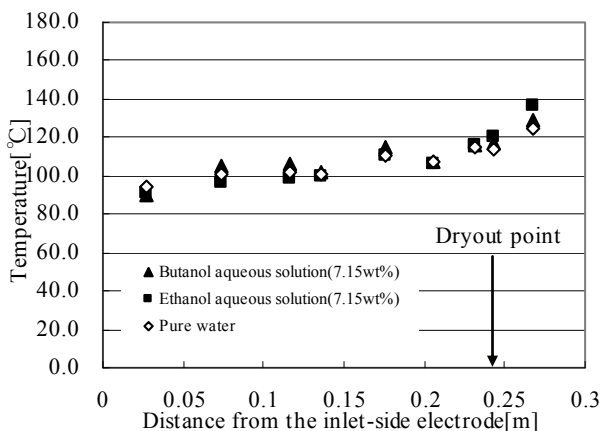
Fig. 11. Time-averaged temperature distribution at the tube surface ( D_m = 1 mm).
