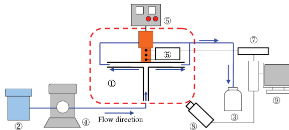
Fig. 17. Experimental apparatus (T-junction mini tube made of quartz glass).
