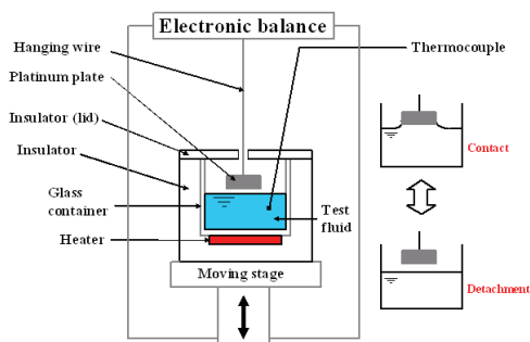
Fig. 3. Experimental apparatus for Wilhelmy's method.
