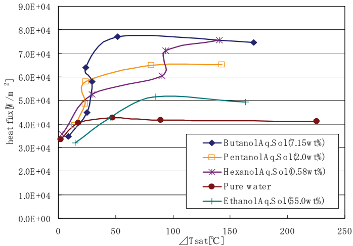
Fig. 15. Boiling curves of all test fluids.
