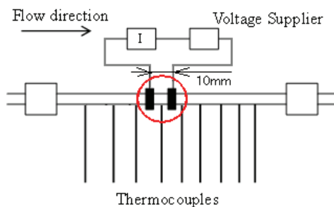
Fig. 12. Test section with the short heating length of D_{in} = 1 mm.
