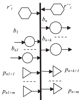
Fig. 4. The common transition schema of E-net representation
