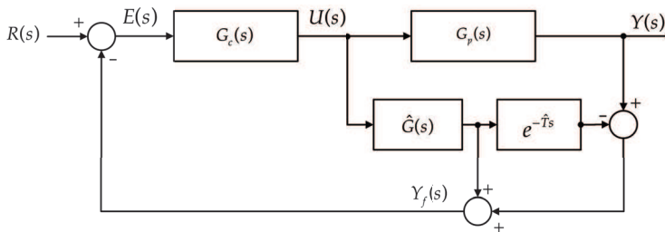
Fig. 4. Smith predictor control structure
