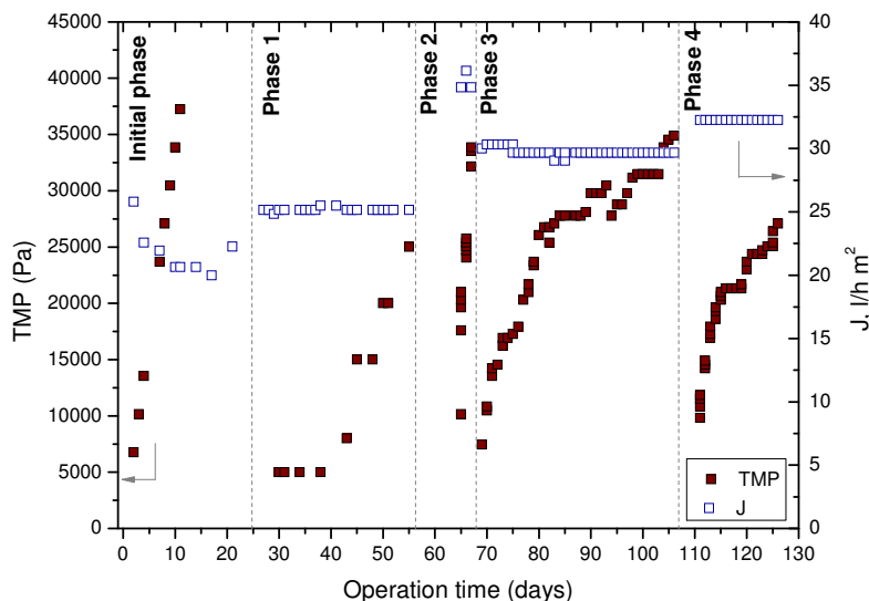
Fig. 11. Transmembrane pressure TMP and permeate flux J evolution with operation time
