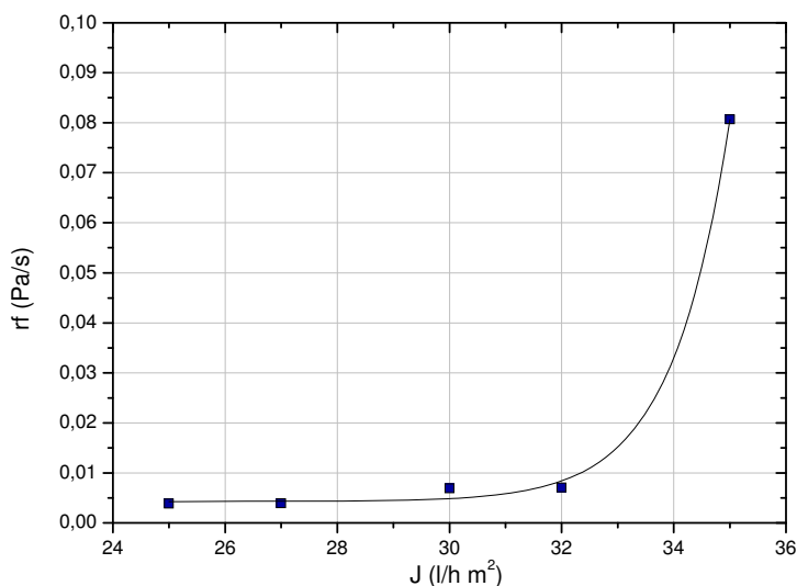
Fig. 12. Fouling rate against permeate flux.
