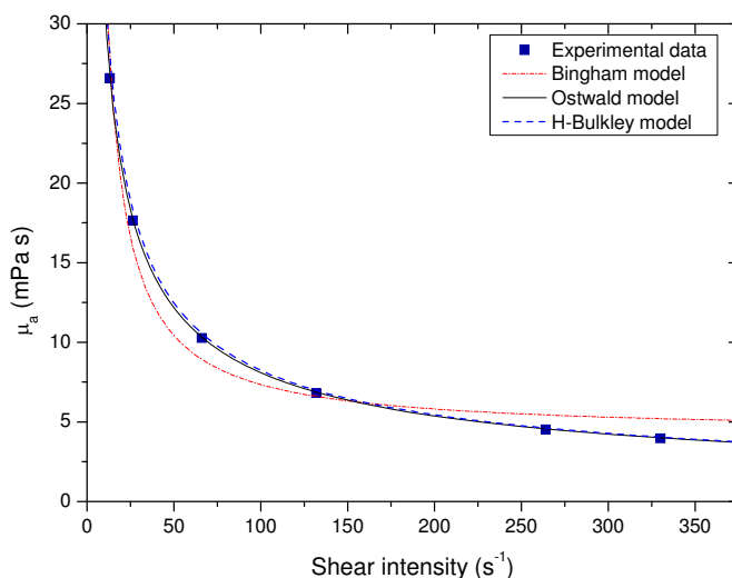
Fig. 8. Apparent viscosity against the shear intensity.
