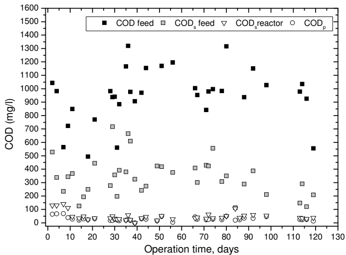
Fig. 13. COD evolution with operation time.
