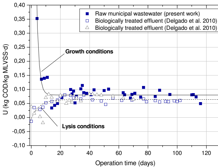
Fig. 5. Evolution of utilisation rate with operation time for MBRs treating different types of feed wastewaters.
