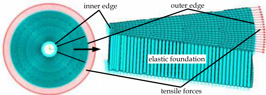
Fig. 28. Second finite element model of the system
