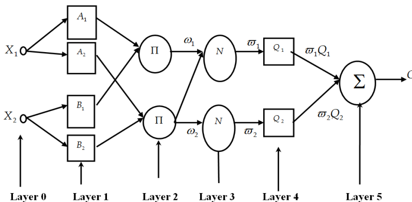
Fig. 8. Two inputs, one output typical ANFIS structure.
