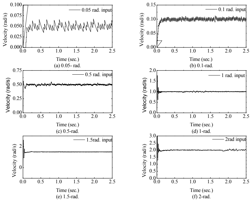
Fig. 5. Samples of positive steady-state velocity responses.
