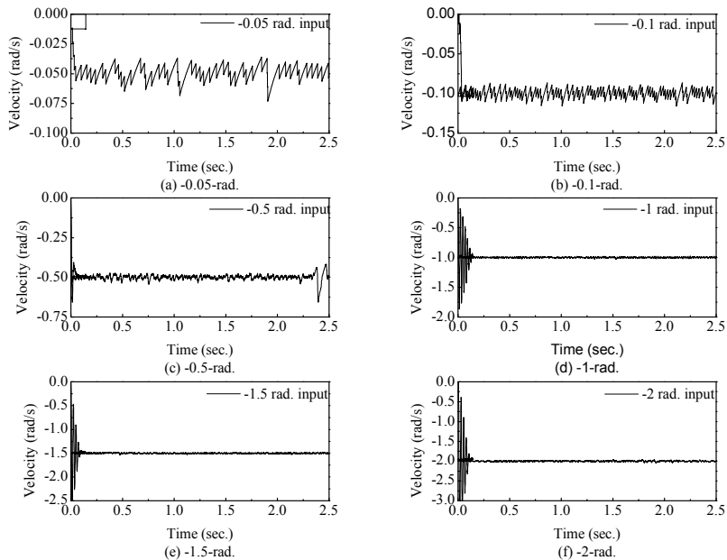
Fig. 6. Samples of negative steady-state velocity responses.
