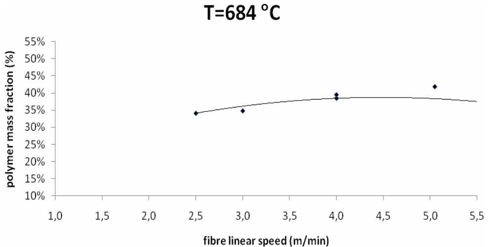
Fig. 9. Polymer mass fraction variation with fibre pull speed for 684 °C oven temperature
