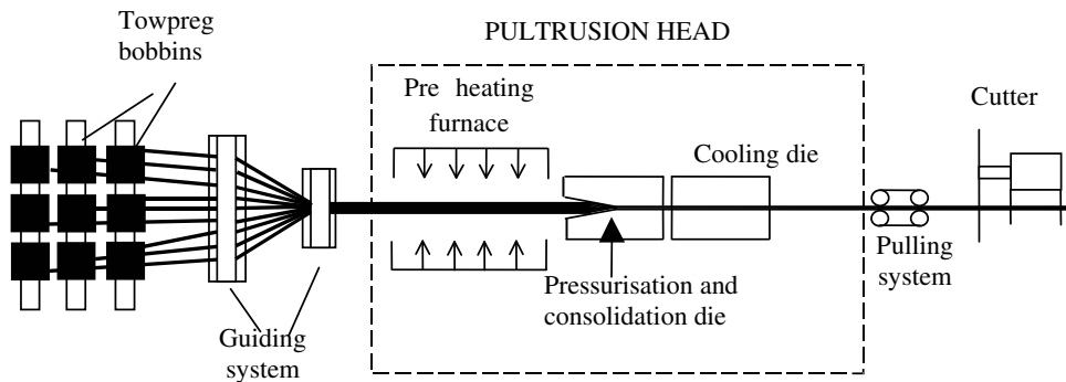
Fig. 14. Schematic diagram of the pultrusion line
