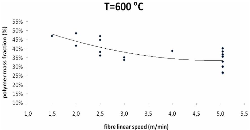
Fig. 7. Polymer mass fraction variation with fibre pull speed for 600 °C oven temperature
