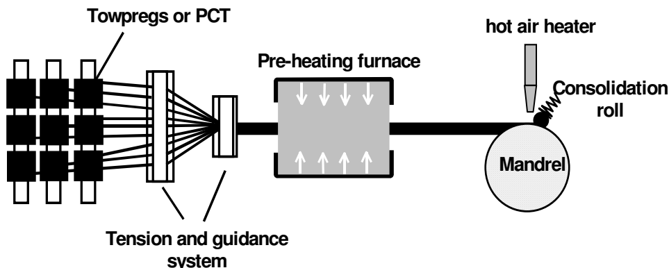
Fig. 13. Schematic representation of the filament winding system
