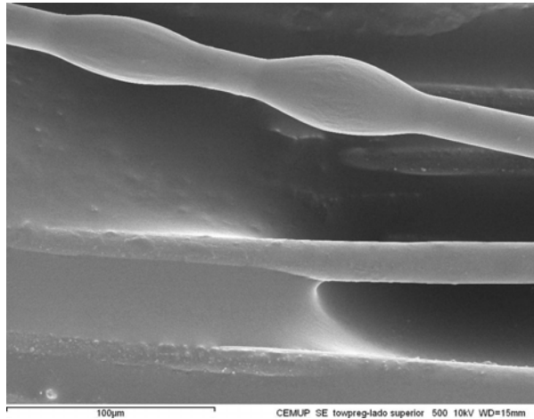
Fig. 11. SEM micrograph of GF/PVC towpreg (magnification of 1000×)
