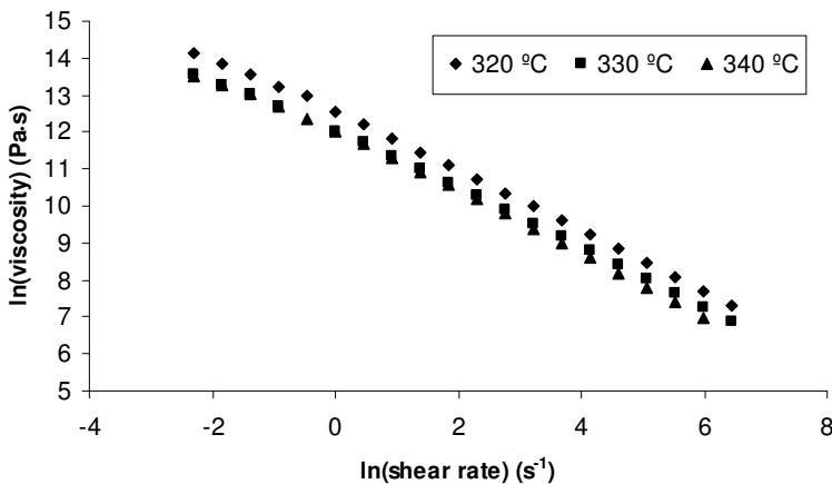
Fig. 4. Dependence of the viscosity on shear rate at different temperatures in a ln-ln scale
