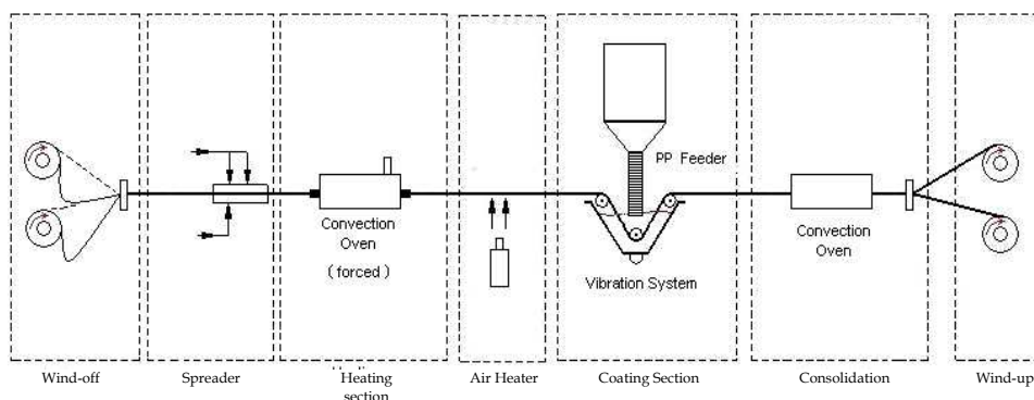
Fig. 1. Schematic diagram of the powder-coating line set-up
