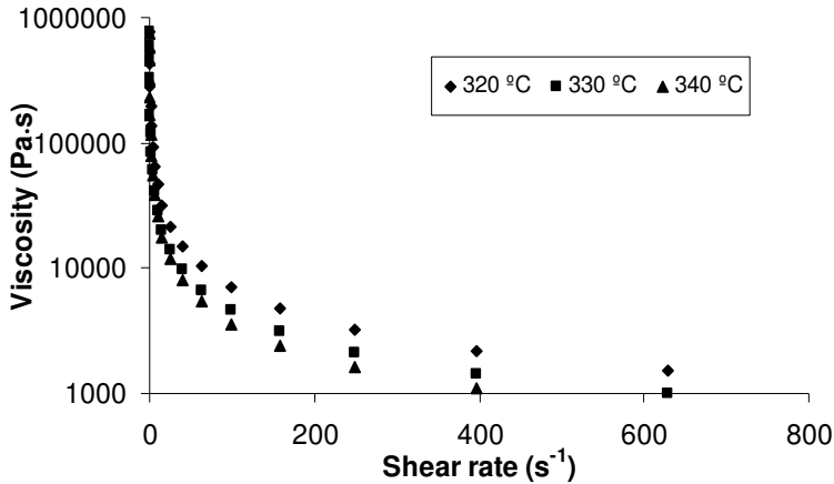
Fig. 3. Dependence of the Primospire® viscosity on shear rate at different temperatures
