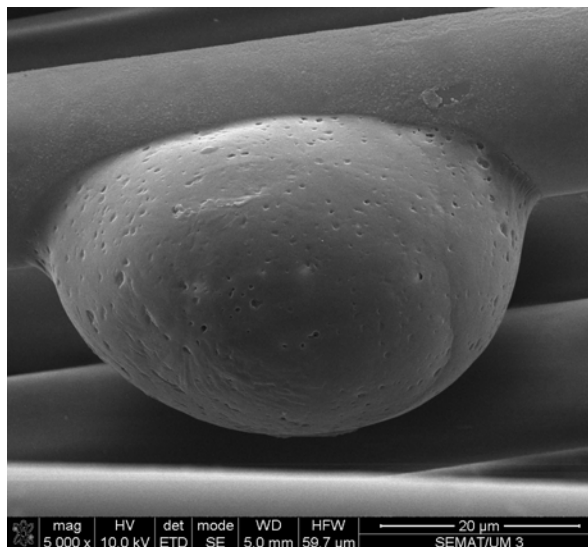
Fig. 10. SEM micrograph of GF/PP towpreg (magnification of 5000×)
