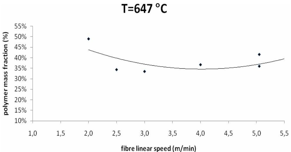
Fig. 8. Polymer mass fraction variation with fibre pull speed for 647 °C oven temperature
