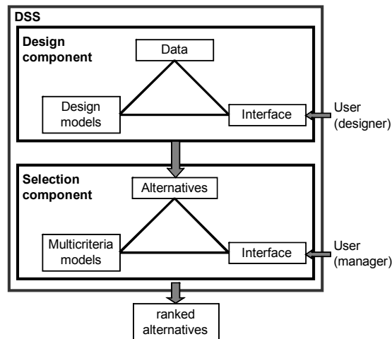
Fig. 1. Conceptual structure of SADREG
