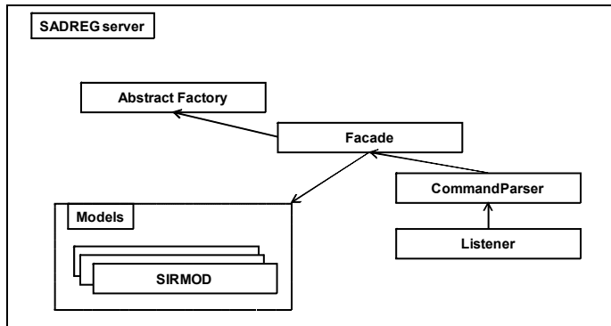
Fig. 12. Models integration on DSS Web server.
