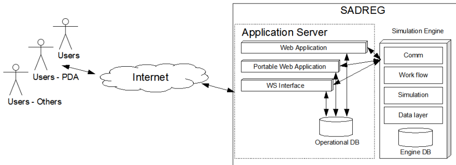
Fig. 9. Abstract system architecture
