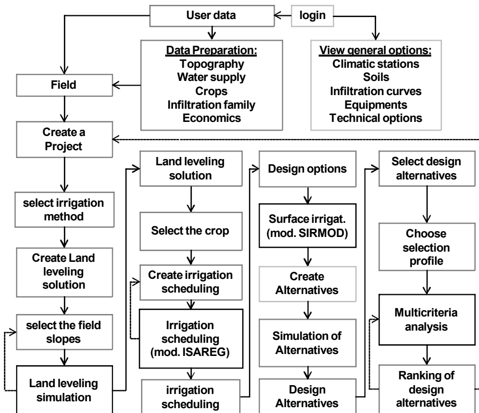
Fig. 13. Data and simulation flowchart
