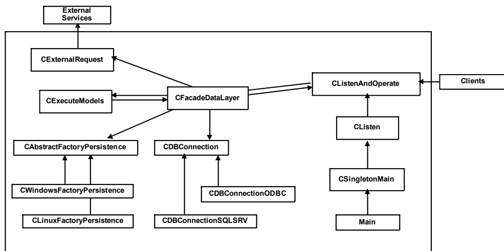
Fig. 10. Architecture of DSS Web Server
