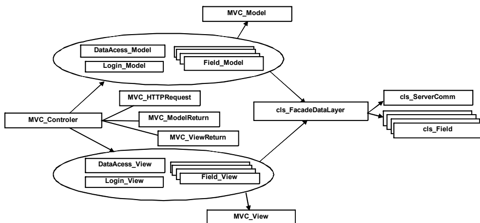
Fig. 11. Architecture of DSS Web Client
