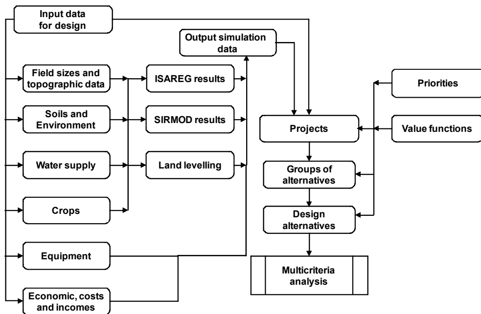
Fig. 2. Data base components in relation with respective data sources and uses in the design process
