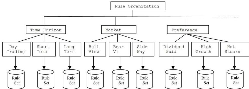
Fig. 2. Knowledge Organization
