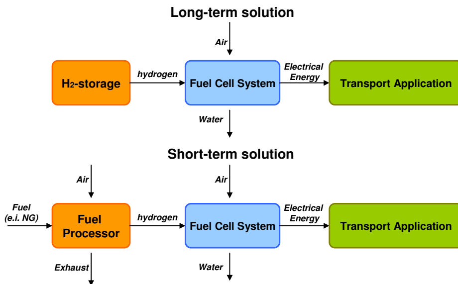
Fig. 17. Fuel options for fuel cell power generation.
