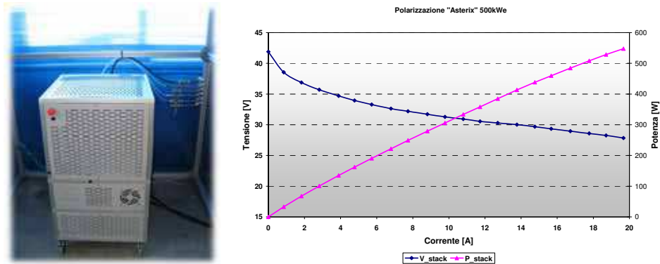
Fig. 26. Polarization curve of a SOFC system with a power of 500 W.
