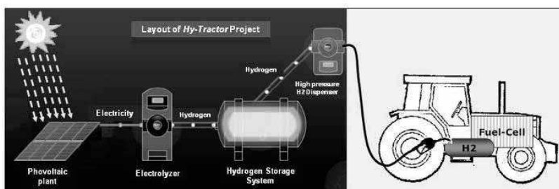
Fig. 20. “Hy-Tractor”: Project layout with photovoltaic plant.
