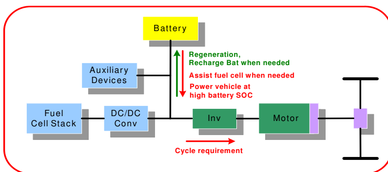
Fig. 16. Fuel Cell Hybrid Electric Vehicle configuration
