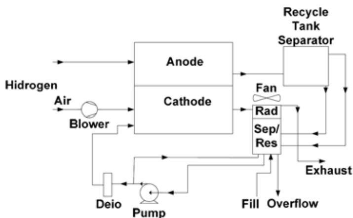
Fig. 22. Schematic diagram of the Fuel Cells System.
