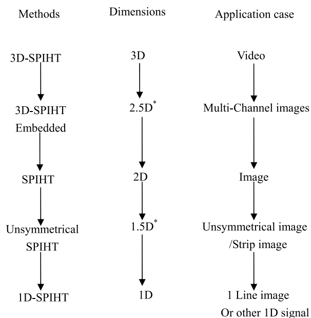
Fig. 6. Family of SPIHT and its derivatives.
