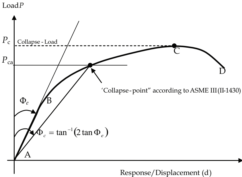
Fig. 3. Load-response history and the collapse-load
