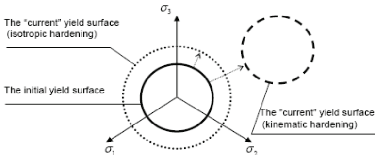
Fig. 5. Isotropic and kinematic hardening behavior on a deviatoric plane
