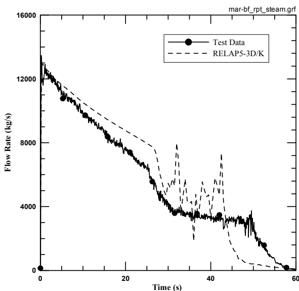
Fig. 2. Comparison of measured and calculated break flow
