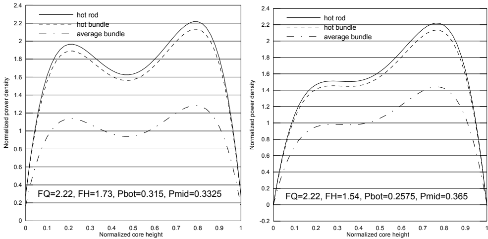
Fig. 23. Sampling of power shapes
