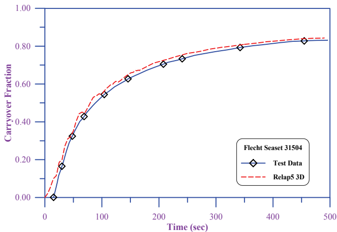
Fig. 10. Comparison of measured and calculated bundle masses
