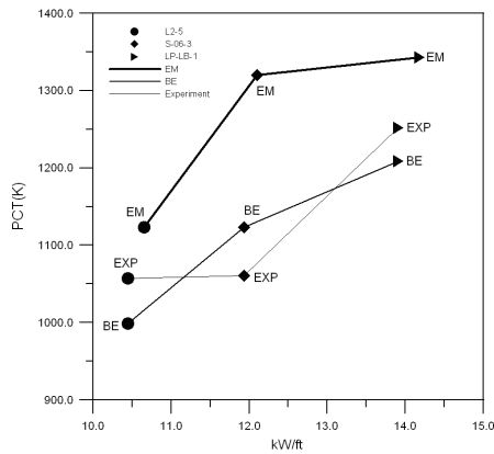
Fig. 17. Conservative trend of PCT calculated by RELAP5-3D/K
