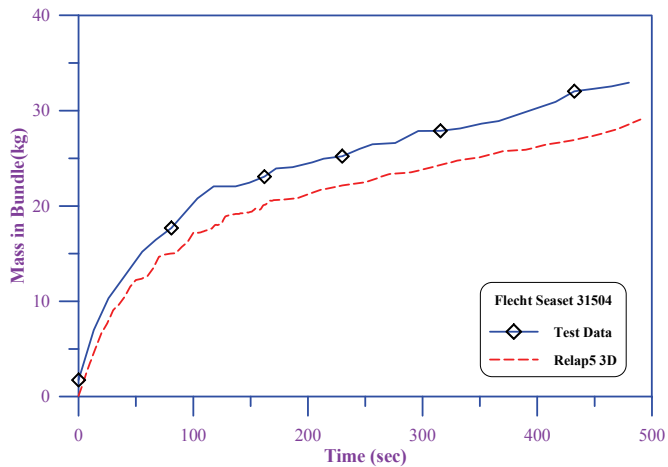
Fig. 9. Comparison of measured and calculated carryover fractions
