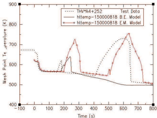
Fig. 20. Comparison of peak cladding temperature of semiscale SBLOCA S-LH-1
