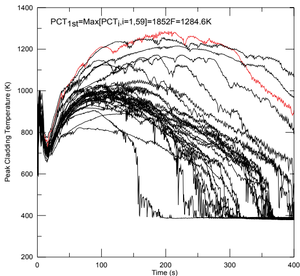
Fig. 25. Calculated PCT of each trial figure
