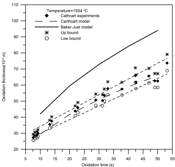
Fig. 1. Oxidation thickness of zirconium 4 (temperature 1504°C)
