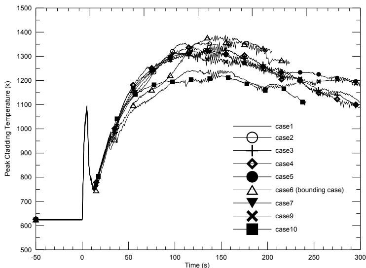
26. Bounding state analysis of PCT
